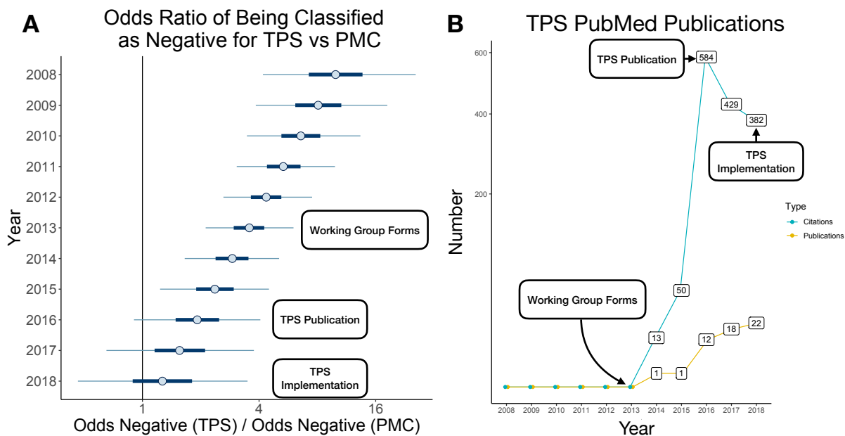
234 Figure 1: Longitudinal differences in negative UC class assignment under each system: A) 235 Odds ratios (OR) and 95% CI (thin line) for assignment of negative UC class between TPS and 236 PMC systems reported yearly in the month of May using the multinomial statistical model; OR 237 of 1 (vertical line) indicates no difference in assignment of negatives between TPS and PMC; 238
