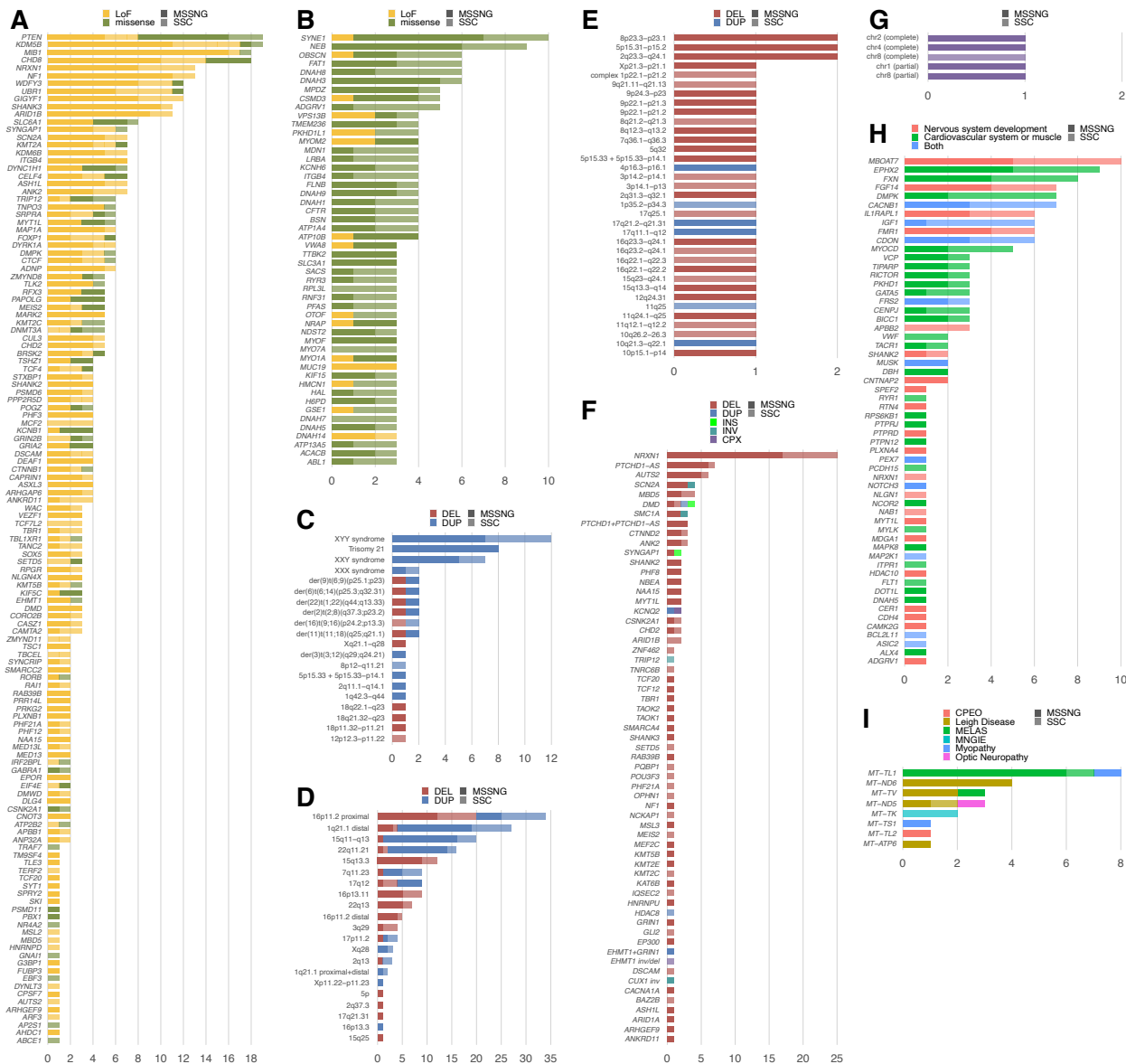
Figure 8: Detailed view of the genomic architecture of rare variants in ASD. Dark versions of a given color represent individuals from MSSNG, while light versions of that same color represent individuals from SSC. (A) De novo or rare inherited (gnomAD allele frequency <10^{-4} ) protein truncating variants (PTVs) and de novo damaging missense variants in genes identified by the TADA+ analysis and/or evaluated as definitive by the EAGLE ASD gene curation process (Schaaf et al., 2020). (B) Recessive (homozygous or compound heterozygous) events. (C) Chromosomal abnormalities. (D) Genomic disorders. (E) Large, gene-rich CNVs other than genomic disorders. (F) Structural variants disrupting the 135 TADA+ genes or other genes with strong evidence for a role in ASD or neurodevelopmental disorders. (G) Uniparental isodisomies. (H) Tandem repeat expansions in enriched gene sets identified previously (Trost et al., 2020). (I) Pathogenic mitochondrial variants. CPEO, chronic progressive external ophthalmoplegia; MELAS, mitochondrial encephalomyopathy, lactic acidosis, and stroke-like episodes; MNGIE, mitochondrial neurogastrointestinal encephalomyopathy.
