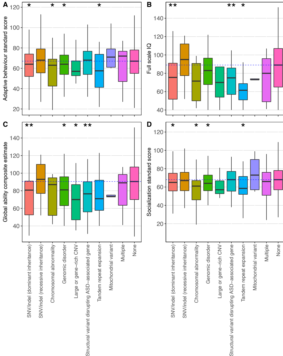
Figure 7: Composite phenotype measure distributions for individuals with ASD having each type of ASD-associated rare variant, or no ASD-associated rare variant (“None”). (A) Adaptive behavior standard score (n=2,787); (B) full-scale IQ (n=1,279); (C) global ability composite estimate (n=1,782); (D) socialization standard score (n=2,765). Asterisks indicate that a given type of rare variant was significantly associated with the phenotype measure (single asterisk: nominally significant with p < 0.05 ; double asterisk: significant after multiple testing correction). The dotted blue line indicates the median of the “None” group.
