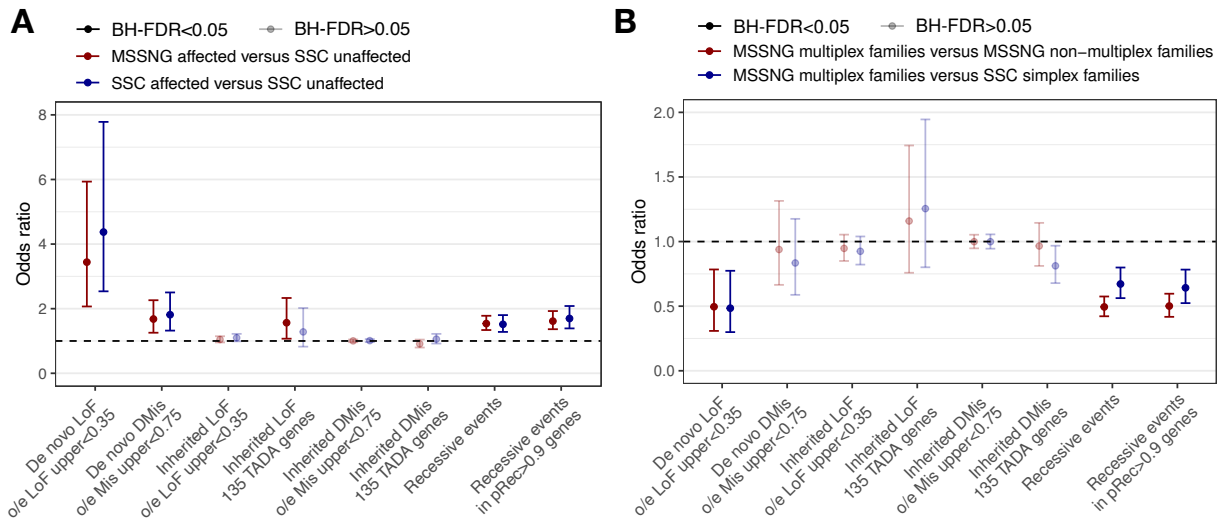
Figure 5: Burden analysis of sequence-level rare coding variants. (A) Individuals with ASD versus siblings without ASD. (B) Individuals with ASD from multiplex families from MSSNG versus those from either simplex families from SSC (defined as families having exactly one individual with ASD and at least one sibling without ASD) or non-multiplex families from MSSNG (defined as families having exactly one individual with ASD and no siblings).
