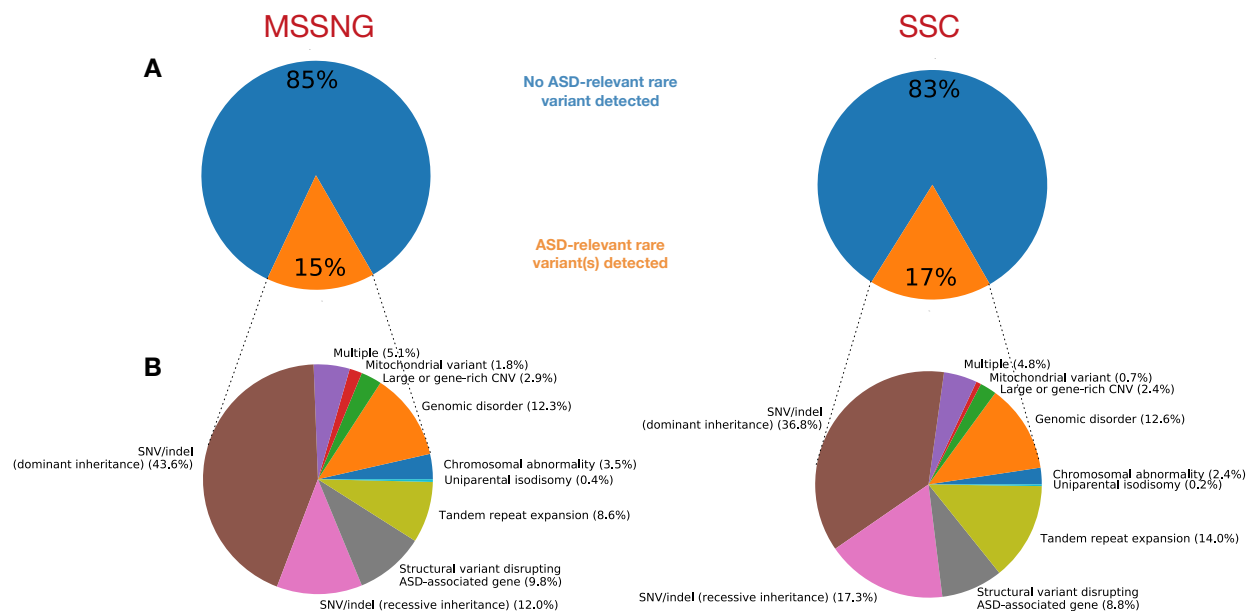
Figure 6: Summary of the genomic architecture of rare variants in ASD. (A) Percentage of individuals with ASD with or without an identified ASD-associated rare variant. (B) Percentage of ASD-associated rare variants in each category. “Multiple” indicates individuals with ASD-associated variants in multiple categories.
