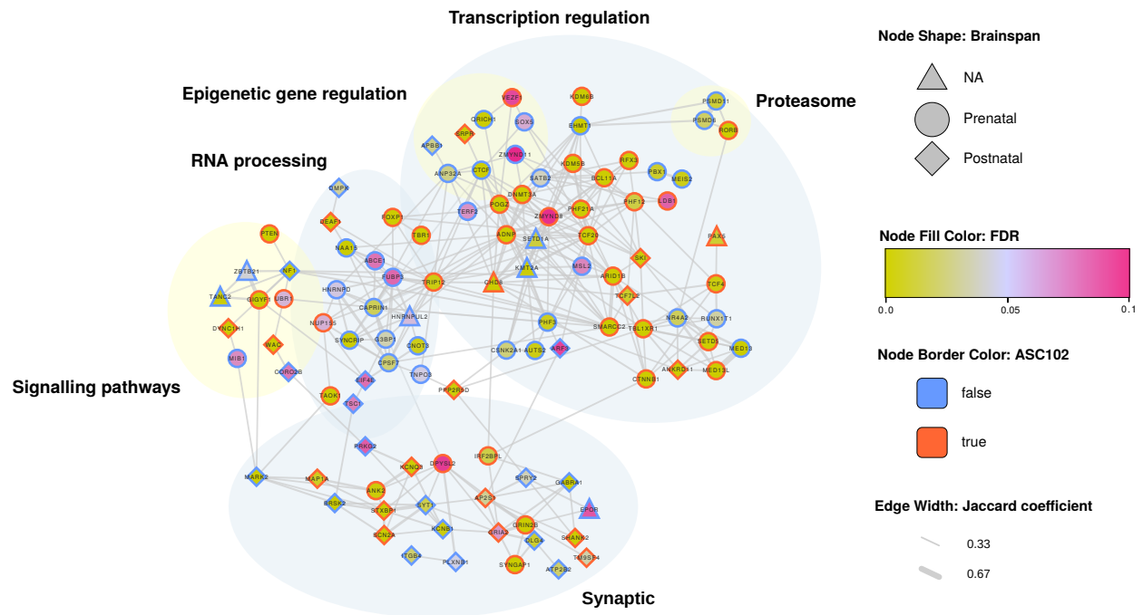
Figure 3: Network diagram of TADA+ genes. Only genes connected to gene networks are shown. Nodes represent genes, and edges represent physical (protein-protein interaction) and pathway interactions between gene pairs. Node shape represents BrainSpan pre/postnatal gene expression (Kang et al., 2011; Miller et al., 2014), and node fill color represents TADA+ FDR (see legend). Red node borders represent genes also identified in the previous ASD TADA+ analysis, while blue borders represent newly identified ASD-associated genes.
