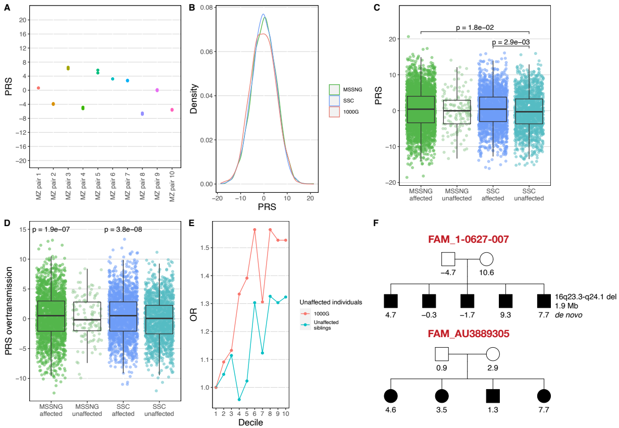
Figure 9: Polygenic risk score (PRS) analysis. (A) Reproducibility in ten pairs of monozygotic (MZ) twins from MSSNG. The PRS of each individual is shown, along with lines depicting the difference in score for each twin pair. (B) PRS distributions in MSSNG, SSC, and 1000G. (C) Comparison between individuals with ASD and their unaffected siblings, stratified by dataset (MSSNG or SSC). Statistically significant differences in means between pairs of groups are indicated; other differences are not significant. (D) Over-transmission of polygenic risk from parents to children in individuals with ASD and their unaffected siblings, stratified by dataset. Values represent the difference between a child's PRS and the mean of his or her parents. If polygenic risk is over-transmitted in a given group, then the mean should be greater than 0. Statistically significant differences from 0 are indicated; means for other groups were not significantly different from 0. (E) Scatterplot showing the odds ratio (OR) of individuals with ASD to unaffected siblings in each PRS decile (decile 1 = bottom 10%, decile 10 = top 10%), relative to the ratio in decile 1, in MSSNG and SSC combined. (F) Pedigrees indicating the PRS for each individual in two large multiplex families in MSSNG.
