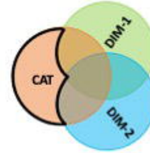
UNIQUE VARIANCE MODEL (STEP 2)
