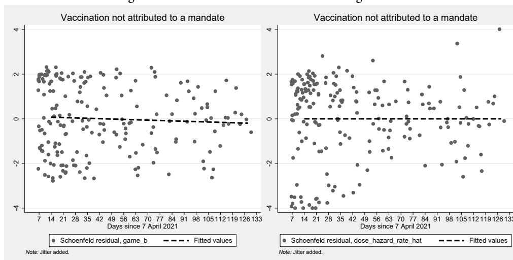
Figure 4: Schoenfeld residuals for the Cox regressions
