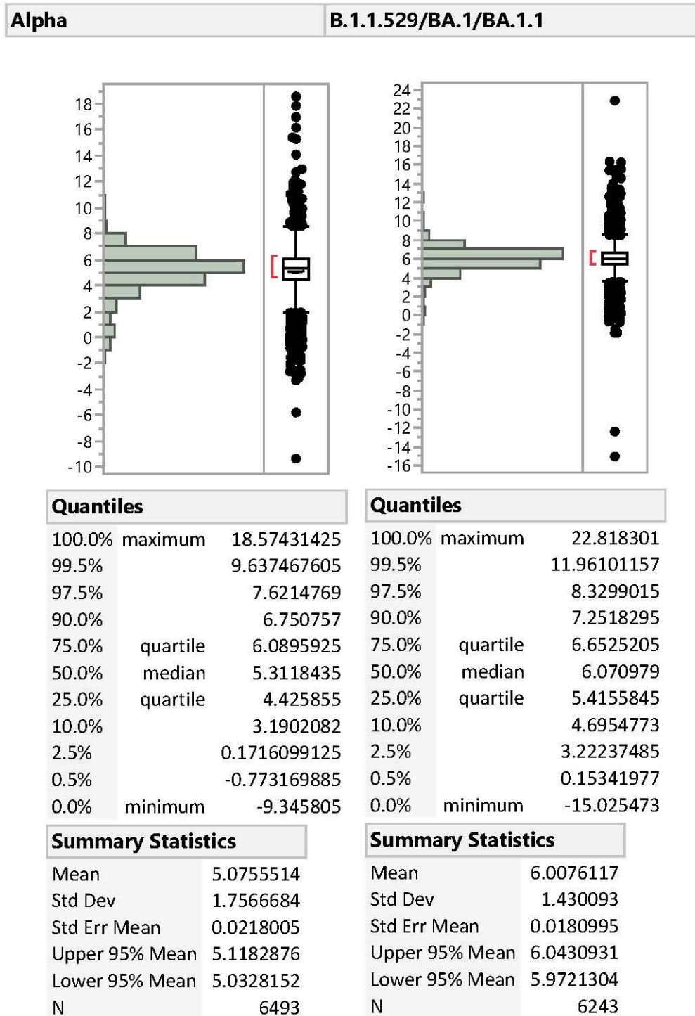
Figure 2: Distribution of Ct value Differences between the S-gene and the average of N and ORF1ab-genes in Alpha and Omicron B.1.1.529/BA.1/BA.1.1 variants
