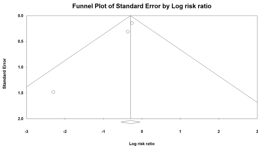
490 Figure 3. the funnel plot of analysis
