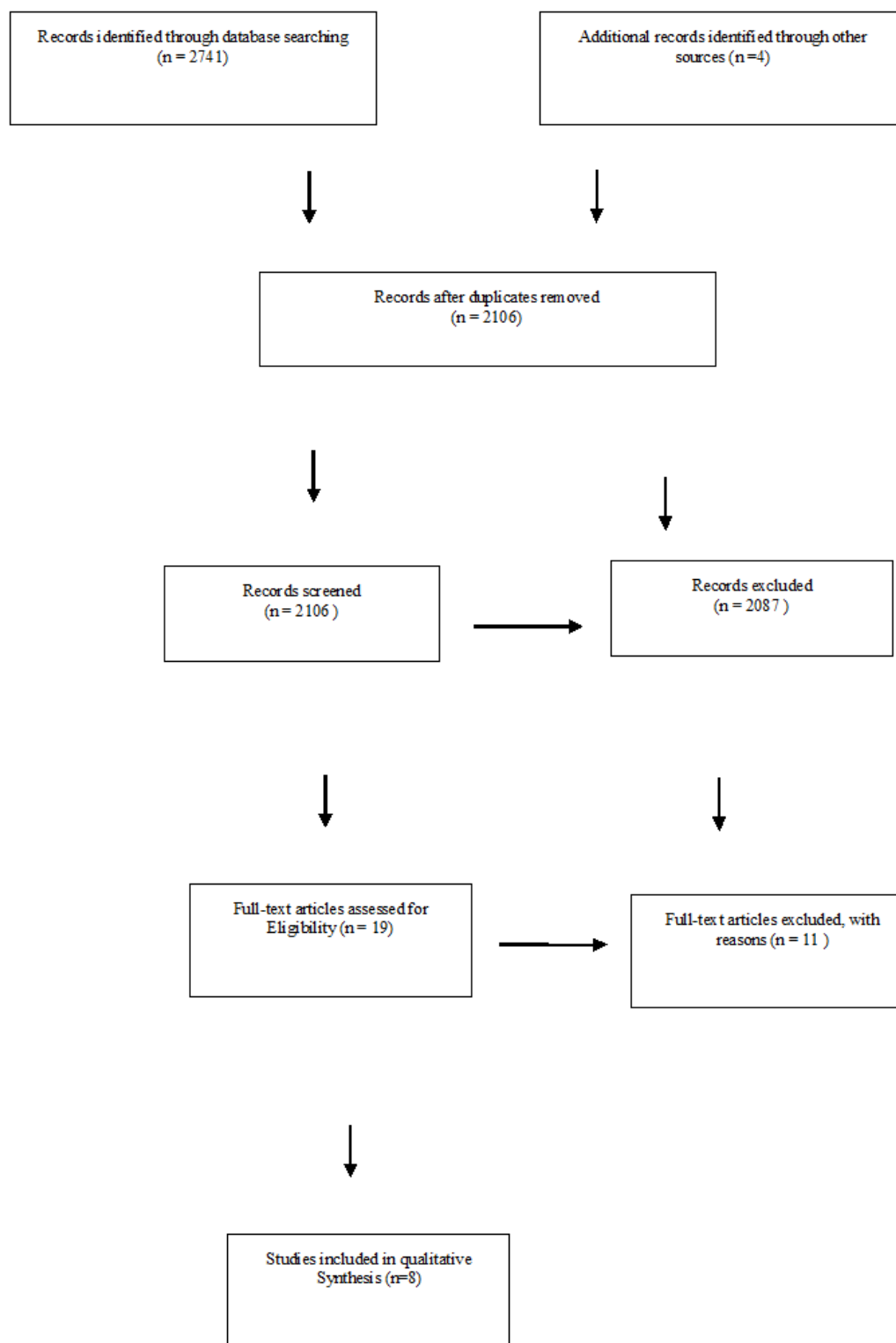
Figure 1: PRISMA diagram
