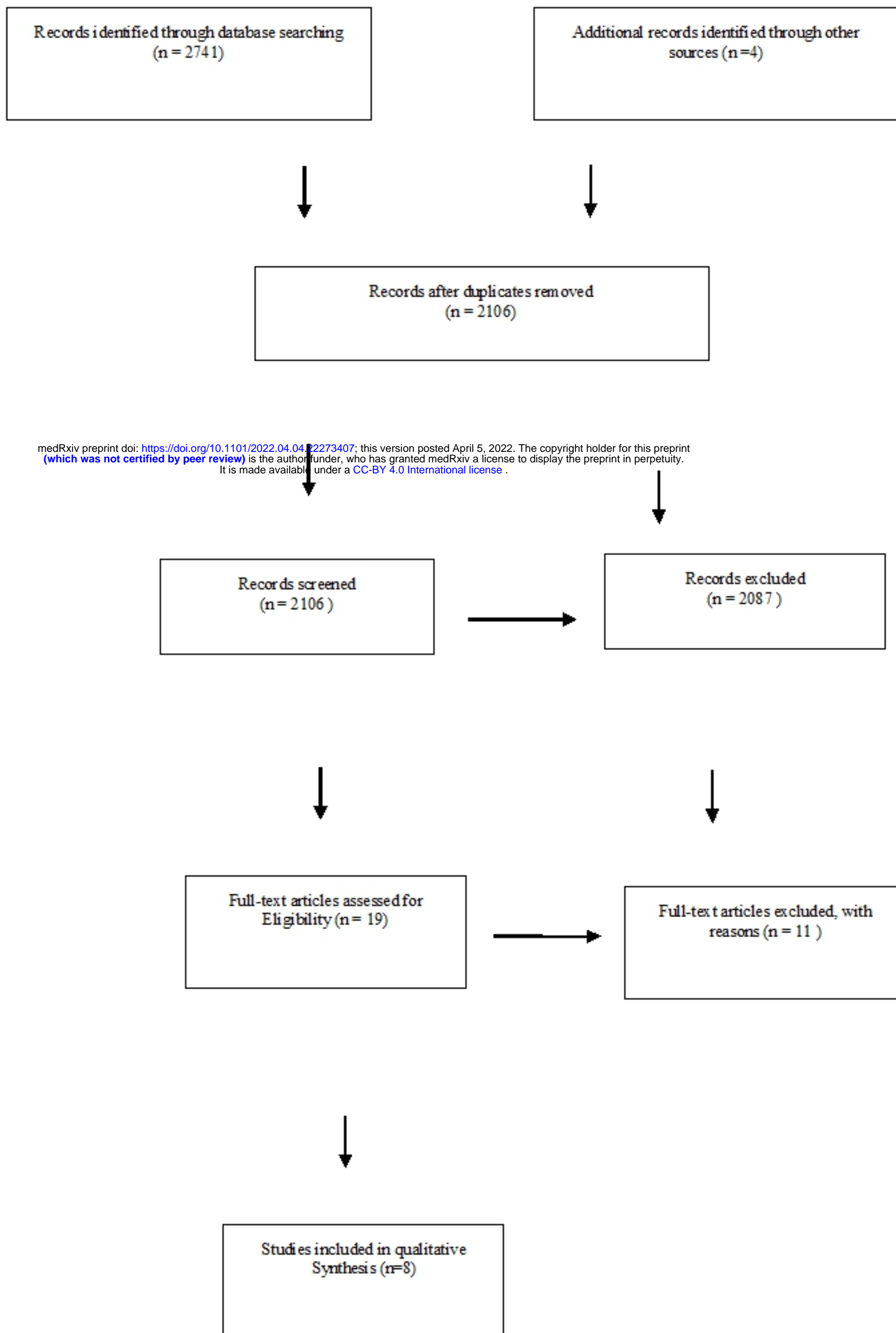
Figure 1: PRISMA diagram
