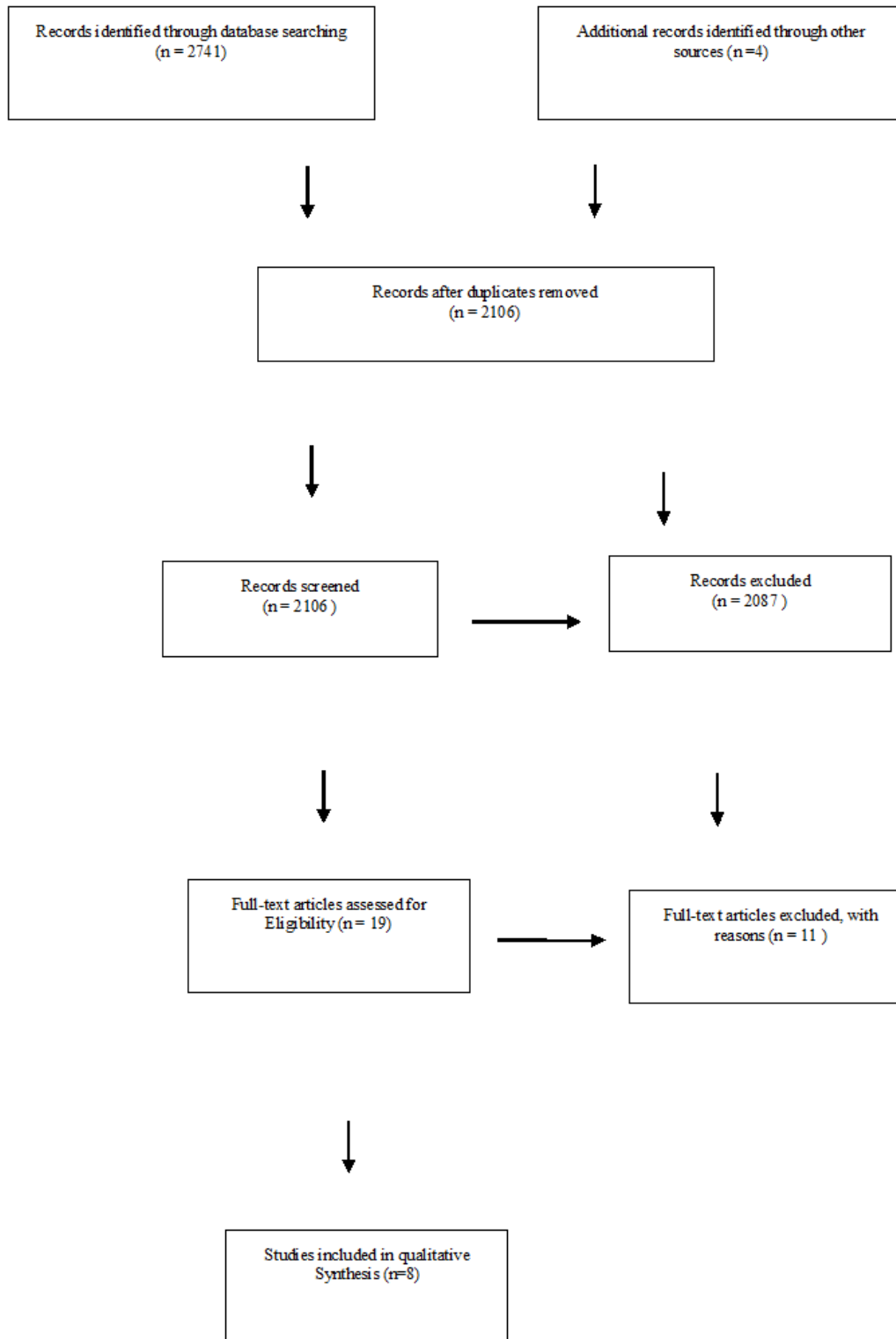
Figure 1: PRISMA diagram
