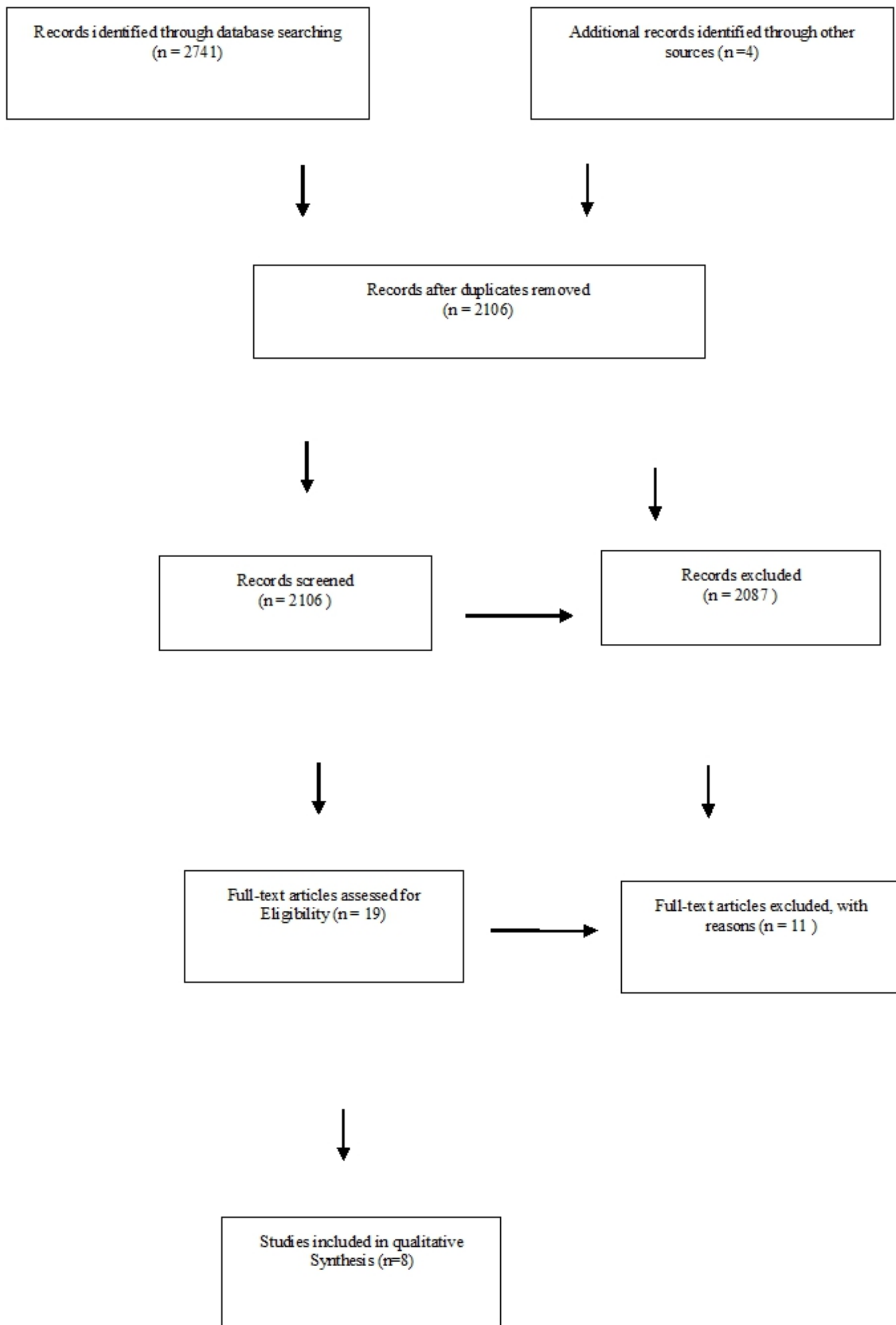
Figure 1: PRISMA diagram
