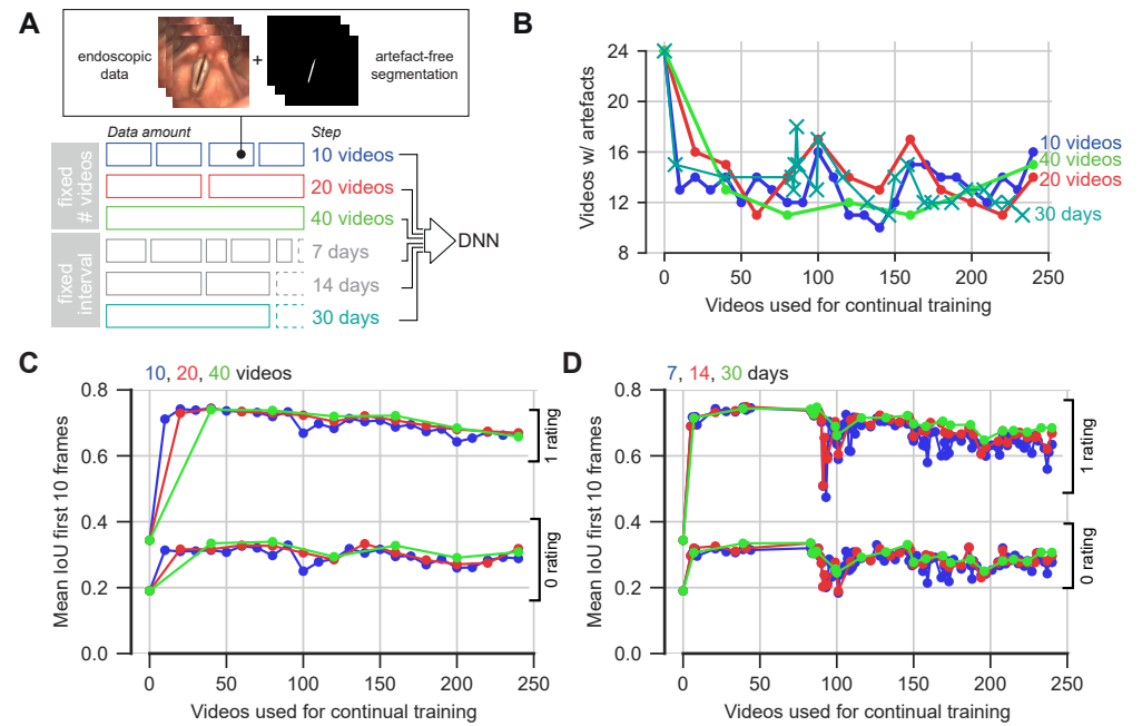
Fig 5. Continual training alleviates segmentation artefacts. A: Continual training strategies. B: Reduction of artefacts depending on continual learning strategy. C: IoU score of the first ten frames of the evaluated data after continual learning with a fixed amount of videos. D: Same as in C, but with a fixed time interval.
