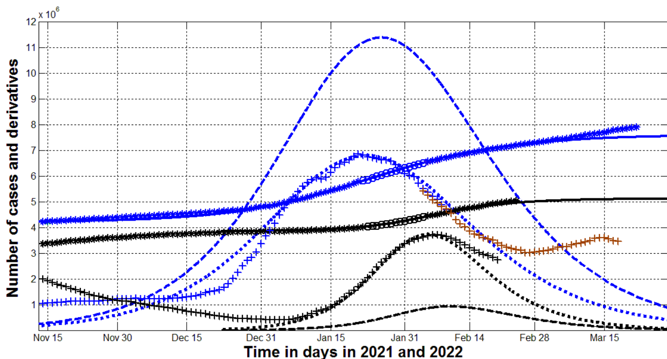
Fig. 1. The omicron waves and further pandemic dynamics in Ukraine and in the whole world. The results of SIR simulations of the 14th wave in Ukraine are shown by black lines. Blue lines represent the 7 th pandemic wave in the world. Numbers of victims V(t)=I(t)+R(t) – solid lines (for the world divided by 60); numbers of infected and spreading I(t) (multiplied by 5 for Ukraine) – dashed; derivatives dV/dt , multiplied by 100 for Ukraine and by 2 for the world) – dotted. “Circles” correspond to the accumulated numbers of cases registered during the periods of time taken for SIR simulations (for the world divided by 60). “Stars” corresponds to V_j values beyond these time periods (for the world divided by 60). “Crosses” show the numerical first derivative multiplied by 100 for Ukraine and by 2 for the world. Black markers correspond to Ukraine ([7], Table 1), blue and brown “crosses” - for the world (different versions of JHU datasets [7], Table 2).
