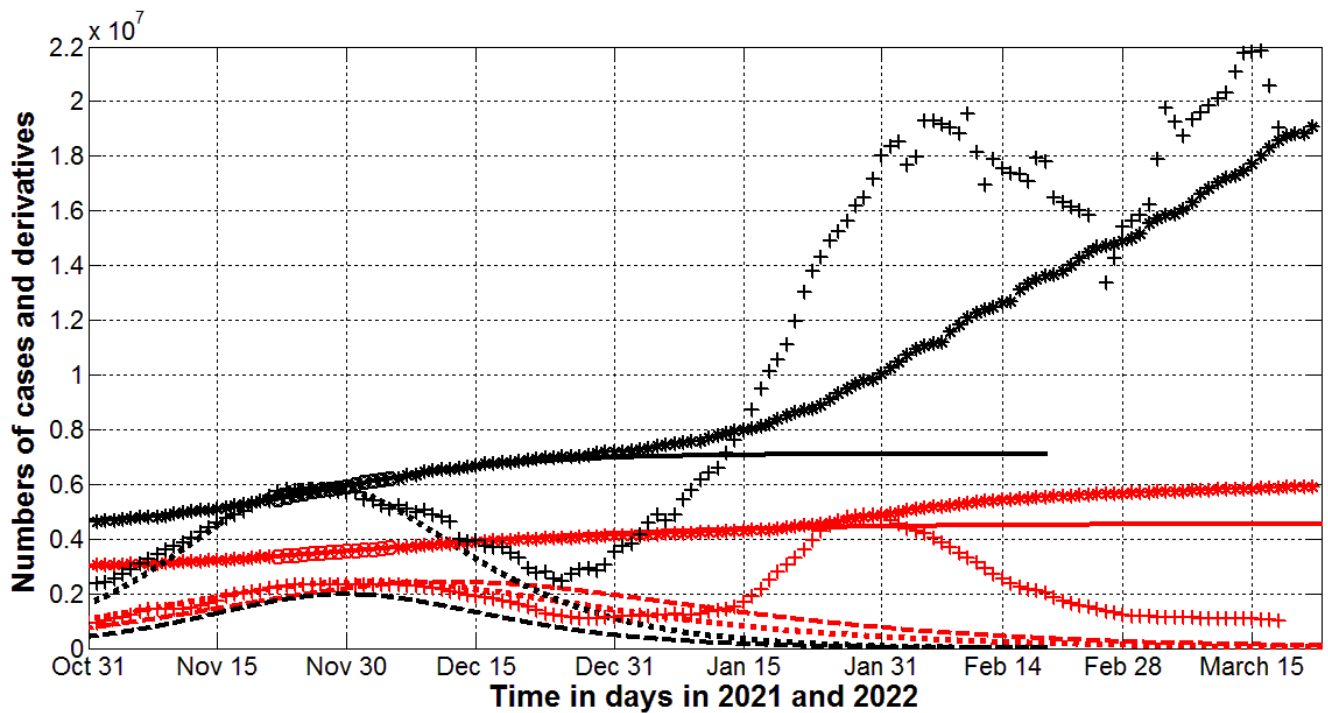
Fig. 2 The COVID-19 pandemic waves in Poland (red) and Germany (black) in 2021 and 2022. The results of SIR simulations of the 4th wave in Poland and the 5th wave in Germany are shown by red and black lines, respectively. Numbers of victims V(t)=I(t)+R(t) – solid lines; numbers of infected and spreading I(t) multiplied by 10 – dashed; derivatives dV/dt (multiplied by 100) – dotted. “Circles” correspond to the accumulated numbers of cases registered during the period of time taken for SIR simulations. “Stars” correspond to V_j values beyond this time period. “Crosses” show the averaged daily number of new cases (calculated with the use of datasets presented in Tables 3, 4 and multiplied by 100).
