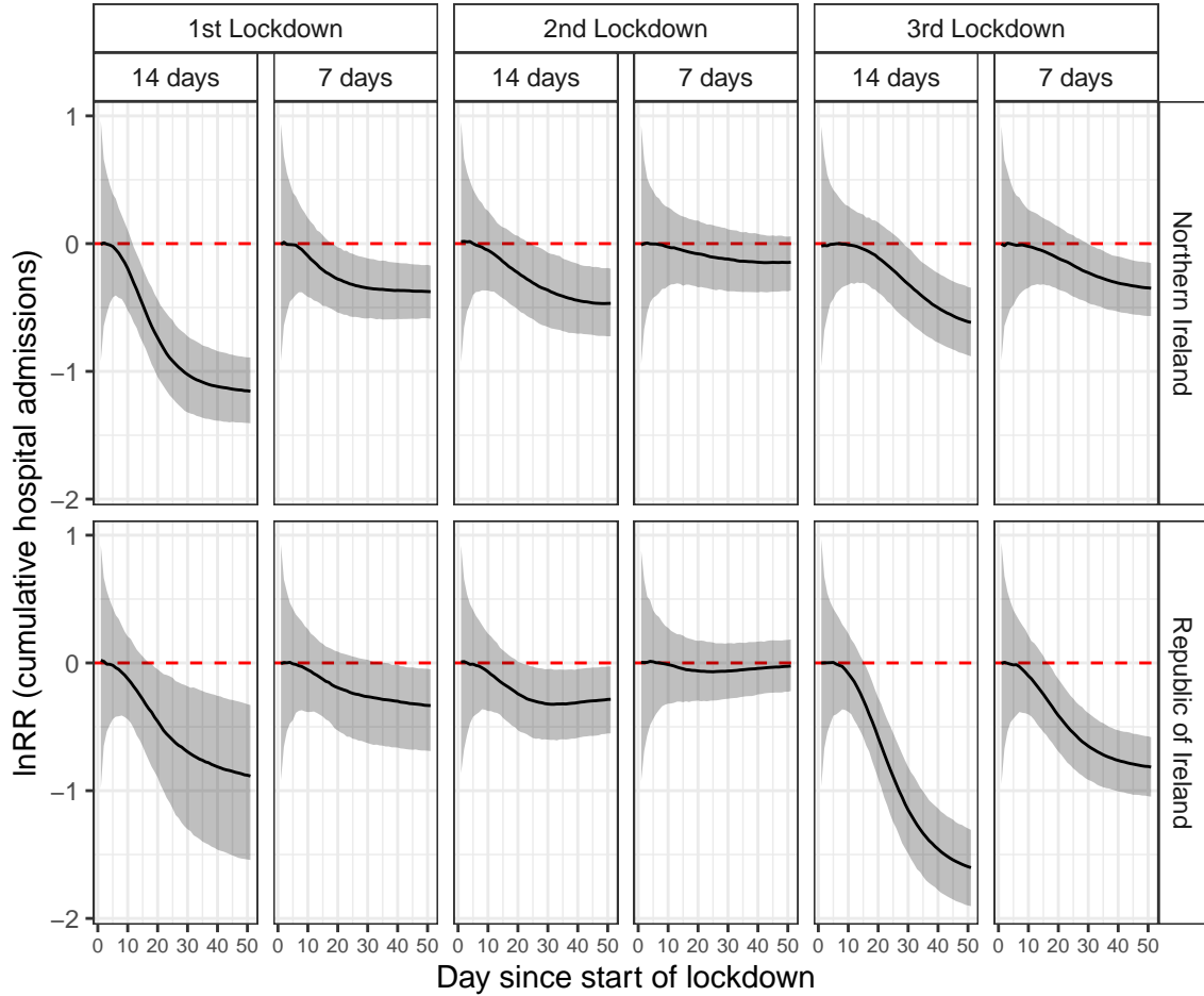
Figure 4: Counterfactual analysis demonstrates the effect of lockdown timing on epidemiological outcomes. The relative difference in cumulative hospital admissions between the counter-factual and factual scenarios is estimated as the log response ratio (lnRR). Shown are the lnRR following the introduction of three lockdowns in Northern Ireland and the Republic of Ireland, assuming that they would have started seven days and 14 days earlier. The black line and grey band indicates the median and 95% predictive interval, respectively.
