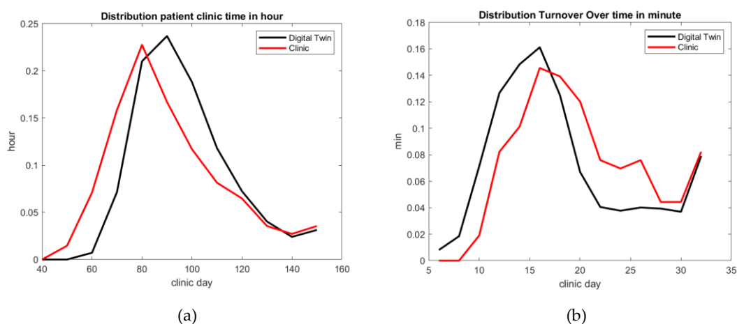
Figure 5: GI Lab 2: comparison of the best fitted digital twin model of patients' total time in the GI lab (a) and turnover overtime (b).
