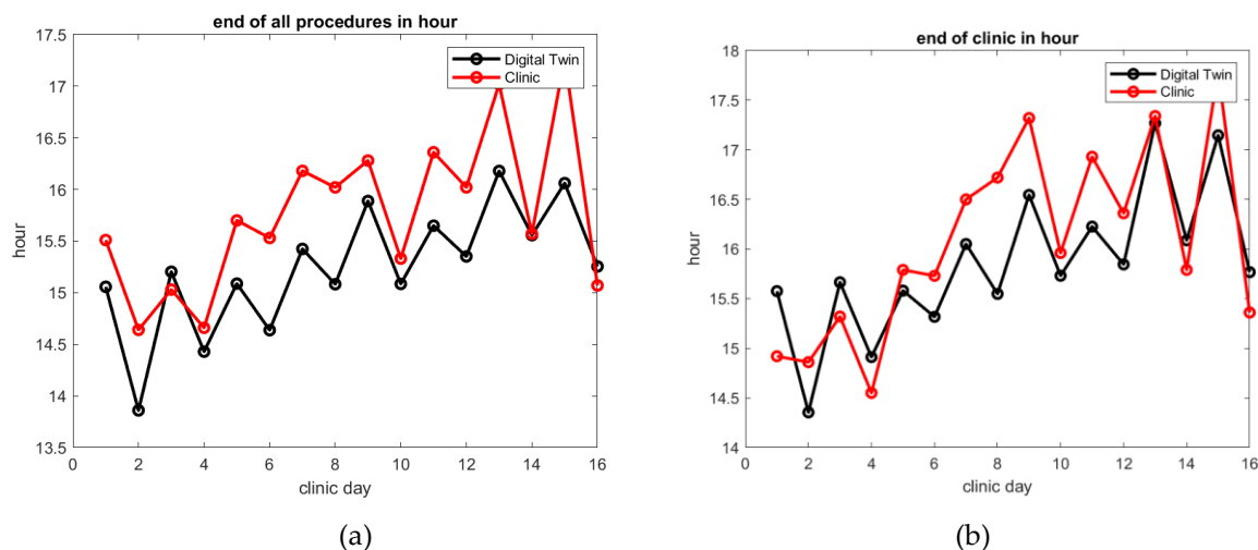
Figure 7: In GI Lab 2, comparison of best fitted digital twin prediction of the end of the last procedure (a) and the end of the clinical day (b). The average difference is 34 minutes for the end of the last procedure and 29 minutes for the end of the clinical day.
