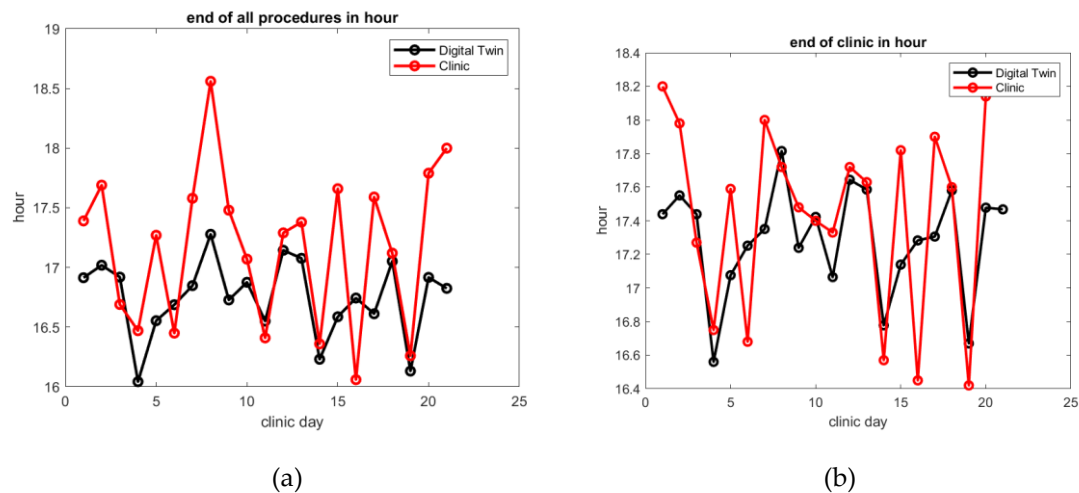
Figure 8: In GI Lab 6, comparison of best fitted digital twin prediction of the end of the last procedure (a) and the end of the clinical day (b). The average difference is 40 minutes only 80% of the time.
