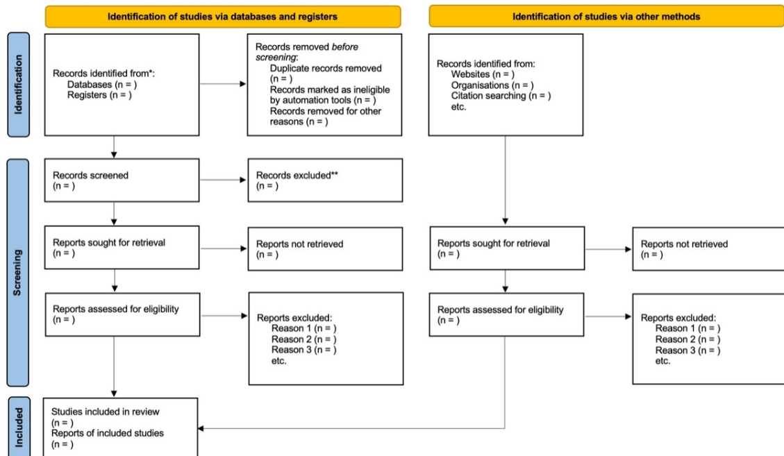
Figure 3. PRISMA flowchart.
