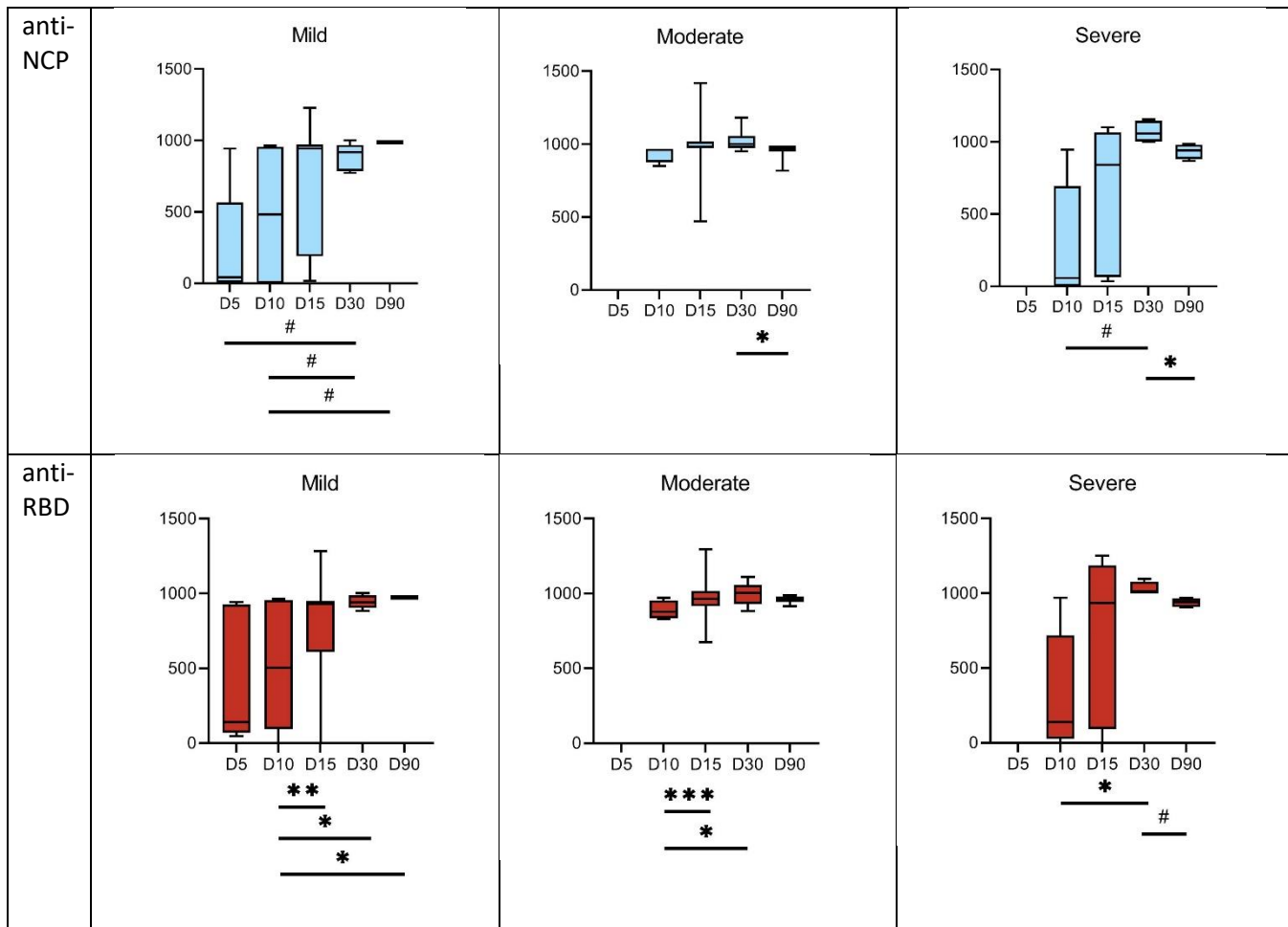
Figure 2. Kinetics of induction of SARS-CoV-2-specific IgG in hospitalized COVID-19 patients; anti-NCP IgG- fraction of IgG specific to nucleocapsid protein of SARS-CoV-2, anti-RBD IgG- fraction of IgG specific to receptor binding protein of SARS-CoV-2, mild – patients treated without assisted respiratory therapy, moderate – patients with limited support of non-invasive assisted respiratory therapy (mask), severe/critical – patients with intensive non-invasive assisted respiratory therapy or invasive mechanical ventilation, days – estimated number of days after onset of infection. Antibodies were identified in blood samples after separation of blood sera by clotting and centrifugation. Microblot-Array testing was applied to quantify IgG level (U/ml). T-test between each time point sample for anti-NCP and anti-RBD IgG titres was applied, # – 0.1 < p < 0.5 ; * – p < 0.05 ; ** – p < 0.01 ; *** – p < 0.001
