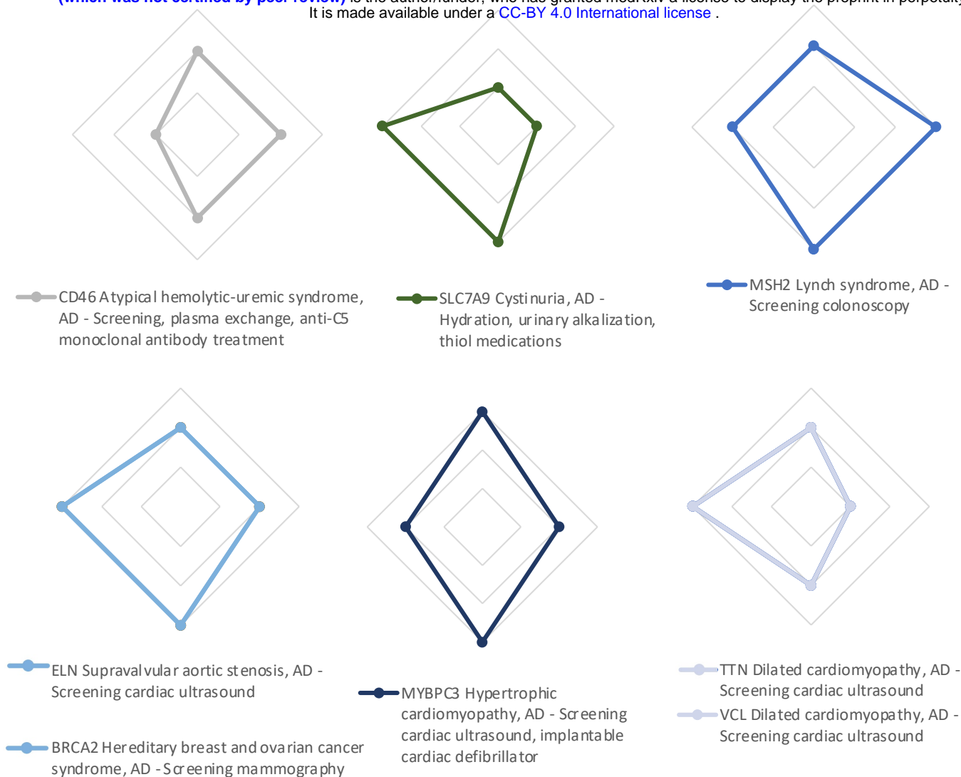
Figure 1: Radar plots that illustrate the pattern of clinical actionability in the specific genes in which unanticipated pathogenic and likely pathogenic variants (PLPVs) were identified. The plot utilizes a modified Semi-Quantitative Metric adapted from ClinGen as described in the text and online methods. As shown in Panel A, the four points of the diamond on the radar graph (starting from the top and moving clockwise with each figure) represent severity of the fully expressed genetic condition, the penetrance or likelihood that the condition will manifest over an individual's lifetime, the effectiveness of the specific intervention shown in the figure and the tolerability of the intervention, i.e., its burden and acceptability to patients. A radar plot with maximum area within the diamond would represent a severe genetic condition that has high penetrance with a highly effective intervention that is particularly acceptable to patients because it is minimally invasive or dangerous. Panel B shows sample clinical actionability radar plots for three genes from the ACMG secondary findings list. Panel C demonstrates clinical actionability of the 14 genes in which PLPVs were identified in the 18 infants with an unanticipated monogenic disease risk. Colors indicate different genes.
