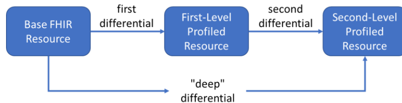
Figure 1. Formulation of the deep differential across multiple levels of profiles (generalizes to any depth).
