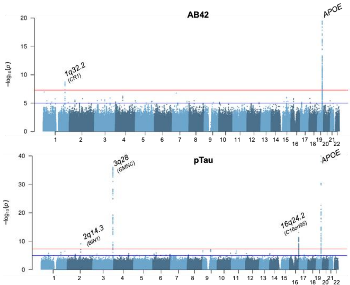
Figure 1. Manhattan plots of the stage 3 GWAs for A \beta 42 and pTau. The y-axes are limited to visualize the non-APOE loci. The lowest p-values for APOE are 4.07 \times 10^{-355} and 3.74 \times 10^{-94} for A \beta 42 and pTau, respectively.
