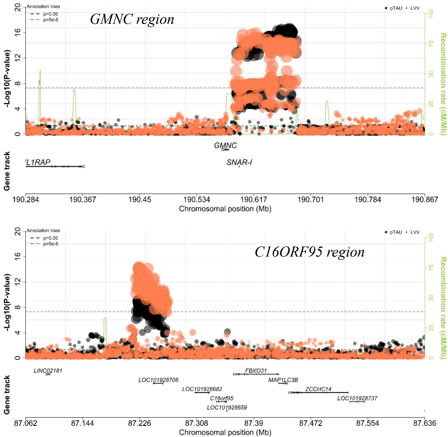
Figure 2. LocusZoom plots showing variant association results for GMNC and C16orf95 loci. In black the pTau association signals of this study, and in orange the lateral ventricular volume (LVV) association signals observed in other studies.
