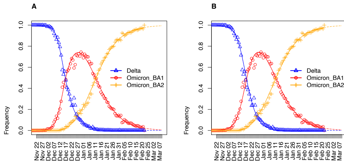
Figure 1. Frequencies of Delta and Omicron from November 22, 2021 to March 9, 2022 estimated using the Three-GT model (A) and the One-GT model (B). Triangles, circles, plus signs represent the frequencies of Delta, Omicron BA.1, and BA.2, respectively. Solid lines indicate the maximum likelihood estimates of frequencies of Delta (blue), Omicron BA.1 (red), and Omicron BA.2 (orange). Dashed lines from February 23, 2022 to March 9, 2022 indicate predicted frequencies of Delta (blue), Omicron BA.1 (red), and Omicron BA.2 (orange). Dotted lines show the upper bound and lower bound of 95% confidence intervals of estimated and predicted frequencies for Delta (blue), Omicron BA.1 (red), and Omicron BA.2 (orange).
