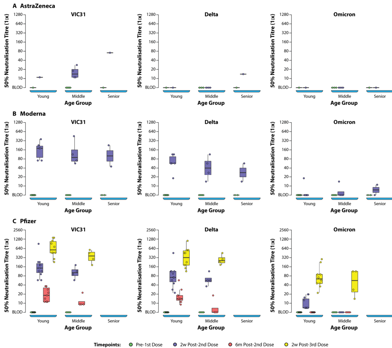
466 Figure 3: Box Plots Showing NT 50 Values Against SARS-CoV-2 Variants of Concern Assessed 467 by Age Group
