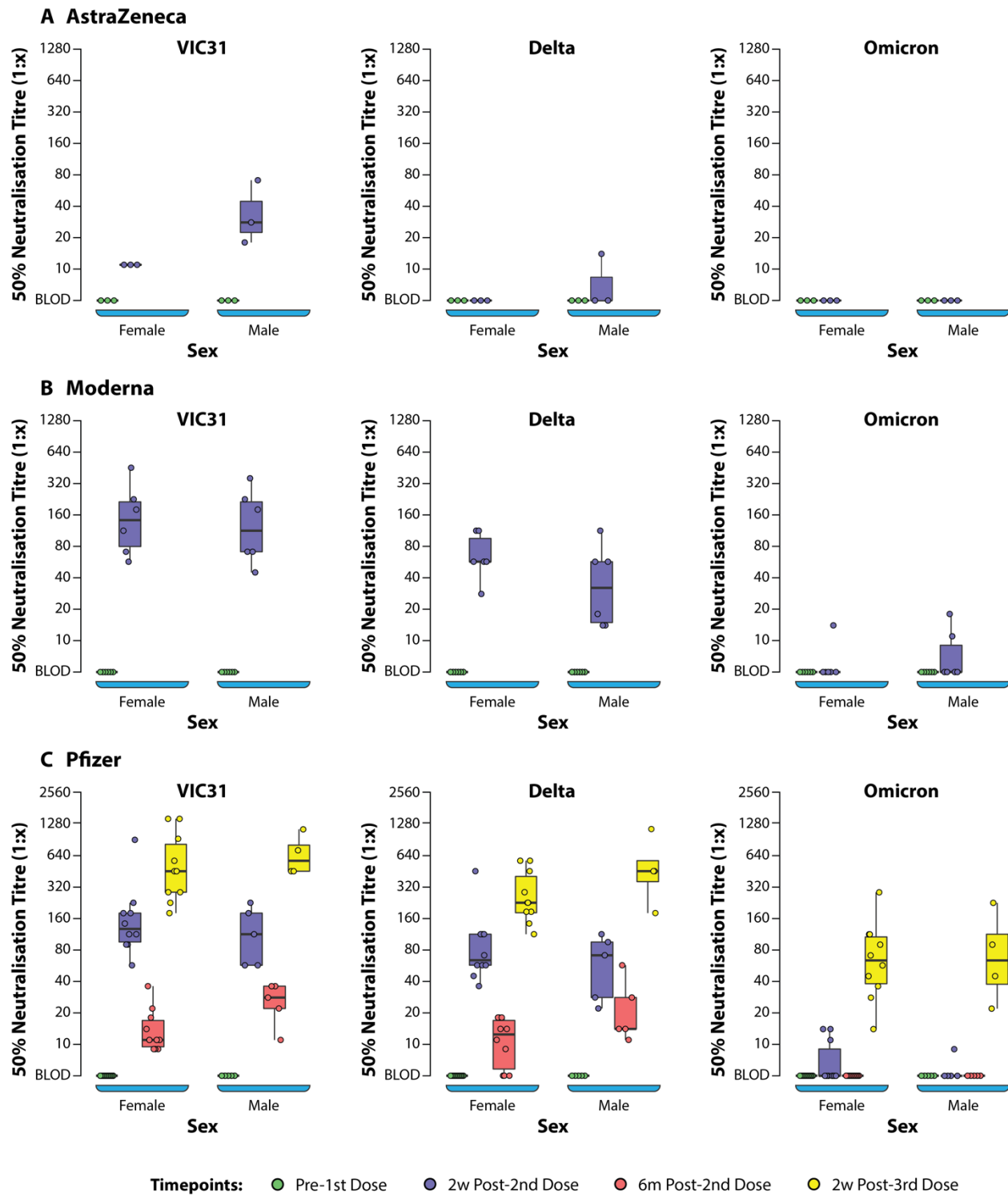
457 Figure 2: Box Plots Showing 50% Neutralization Titres (NT 50 ) Against SARS-CoV-2 Variants 458 of Concern Assessed by Sex of Donors
