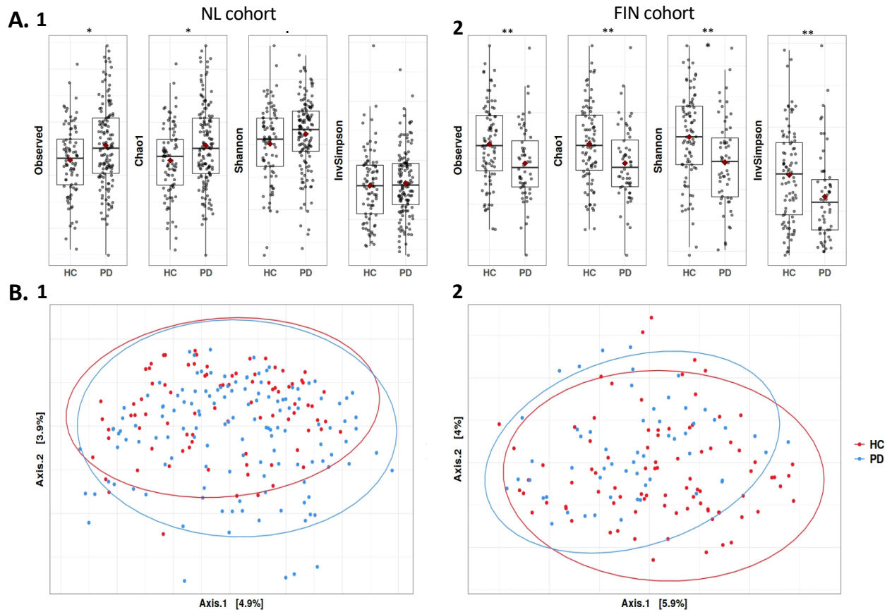
Figure 1. Intra-sample (alpha diversity) and inter-sample differences in microbial community structure between PD and HC with each point representing one sample. A) Alpha diversity indices indicate increased intra-sample diversity in PD in 1) the NL cohort, whereas intra-sample diversity in PD is reduced in 2) the FIN cohort. Univariable, uncorrected (Mann-Whitney U test) p-values are 0.016, 0.016, 0.060 and 0.56 for the NL cohort and 4.3E-03, 4.2E-03, 7.8E-04 and 3.9E-03 for the FIN cohort for, respectively, observed richness, Chao1, Shannon and Inverse Simpson. B) Inter-sample differences in microbial community structure were visualized using a principal component analysis of the Aitchinson distance, indicating a statistically significant differences between PD and HC with p=6.4E-03 and p=4.0E-04 for 1) the NL cohort and 2) the FIN cohort, respectively. Sample sizes: 136 PD and 85 HC for the NL cohort and 56 PD and 87 HC in the FIN cohort. p < 0.1 ; * p < 0.05 ; ** p < 0.01 ; *** p < 0.001 ; NL cohort, Dutch case-control cohort; FIN cohort, Finnish case-control cohort; PD, Parkinson's disease; HC, healthy control.
