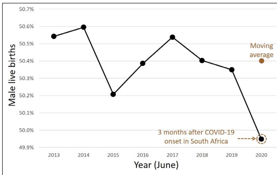
129 Fig 2. Proportion of male live births during the month of June from 2013-2020.
