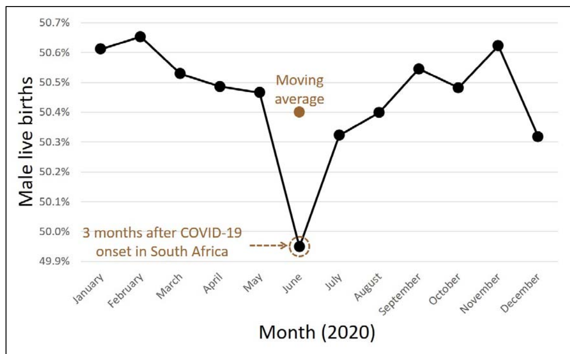
125 126 Fig 1. Monthly proportion of male live births in 2020.
