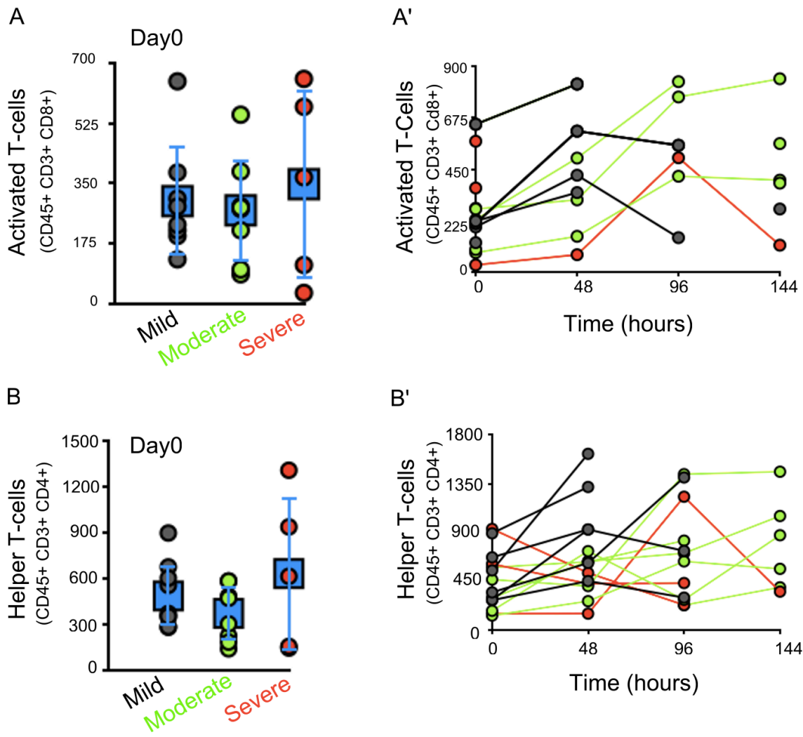
Figure 2: T-cells numbers are not different in COVID-19 patients with varying disease severity
