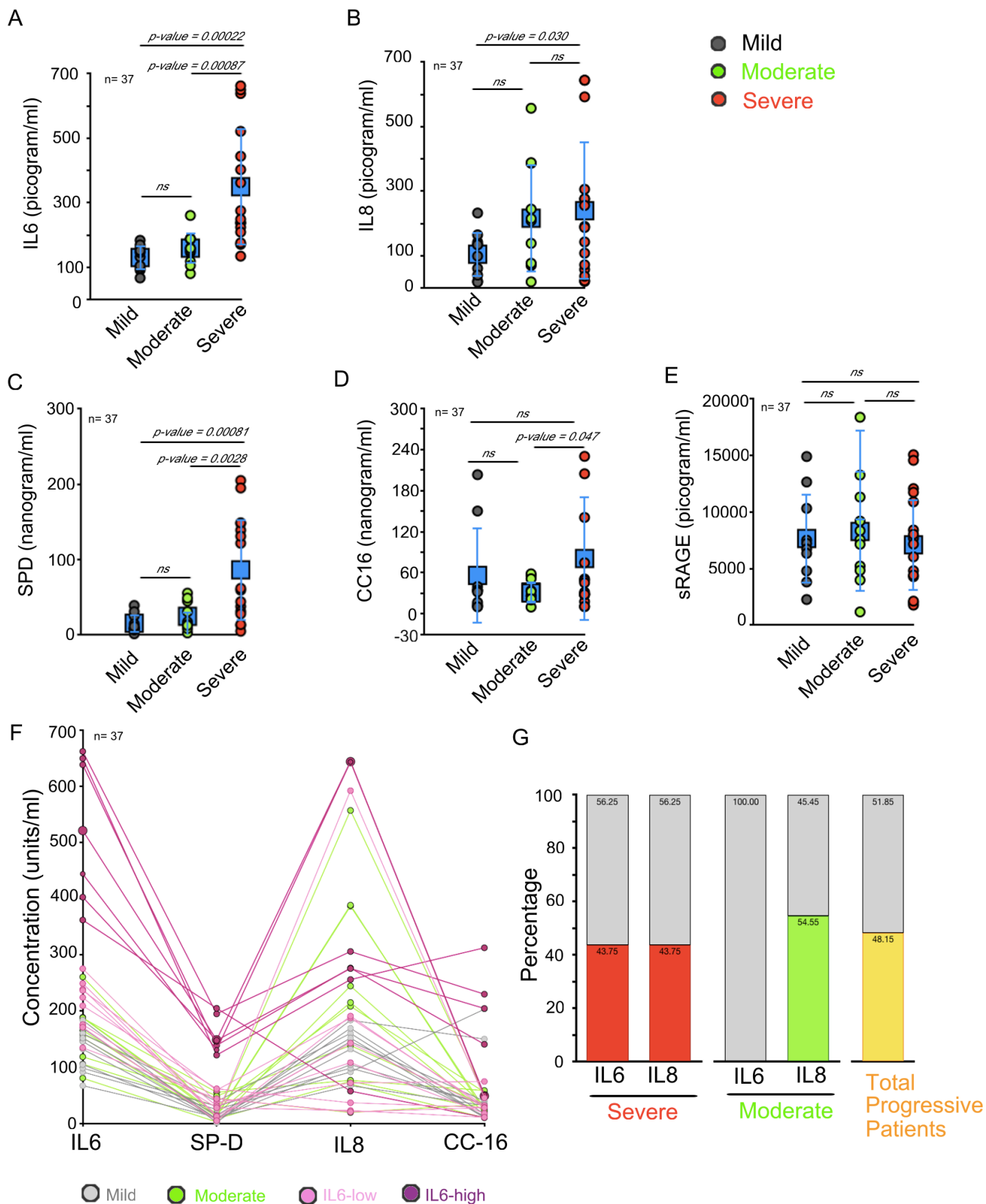
Figure 6: IL6 and IL8 can be used as early markers of progressive COVID-19 disease
