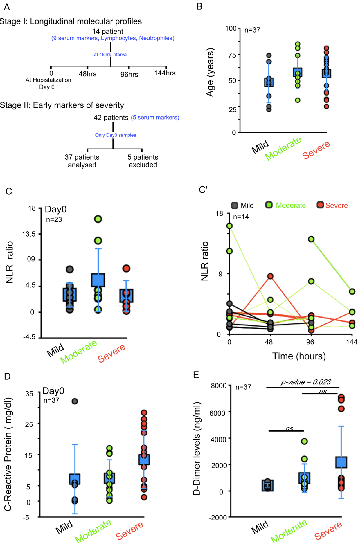
Figure 1: NLR ratio and CRP levels fail to predict disease severity in COVID-19 patients
