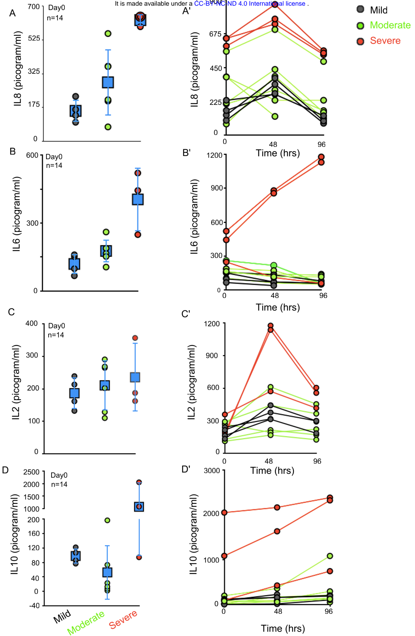
Figure 4: IL2, IL6, IL10 and IL8 are elevated in severe COVID-19 patients.
