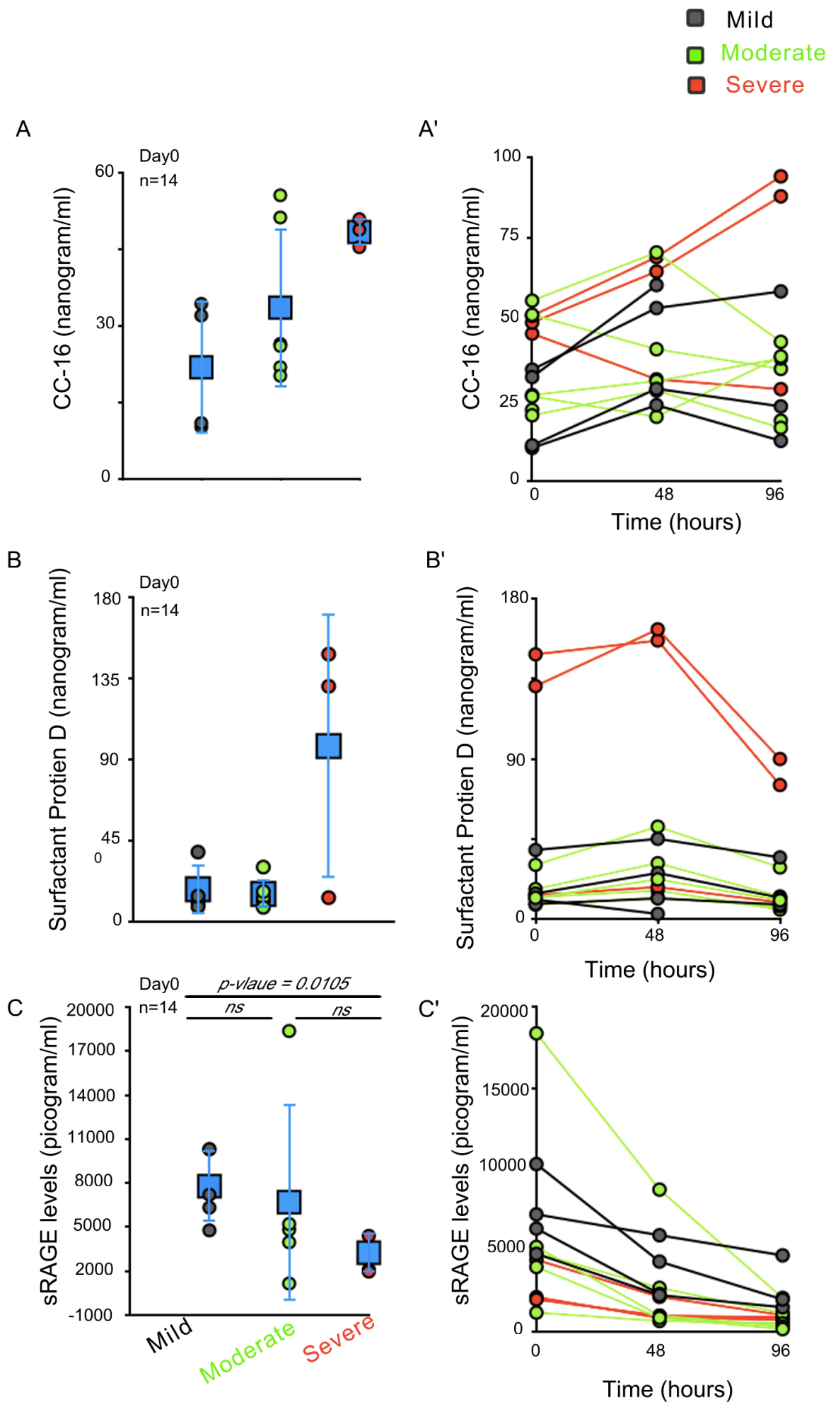
Figure 5: SP-D is upregulated in severe COVID-19 patients unlike sRAGE.
