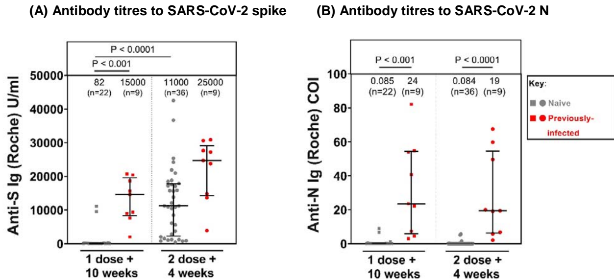
Supplementary Figure 1 | Antibody titres to SARS-CoV-2 spike and nucleocapsid protein in both naïve and previously-infected healthcare workers at 1 dose + 10 weeks and 2 dose + 4 weeks. (A) Antibody titres to SARS-CoV-2 spike protein in naïve and previously infected healthcare workers at 1 dose + 10 weeks and 2 dose + 4 weeks. (B) Antibody titres to SARS-CoV-2 nucleocapsid protein in naïve and previously infected healthcare workers at 1 dose + 10 weeks and 2 dose + 4 weeks. (A-B) Healthcare workers received phlebotomy 10 weeks post 1 st dose (1 dose + 10 weeks) and/or 4 weeks post 2 nd dose (2 dose + 4 weeks). Patients are matched for data measured by PITCH ELISpot and Oxford Immunotec T-SPOT assays. Roche assay was used to determine Antibody (Ig) titres in U/ml for anti-S and cut-off index (COI) for anti-N. At 1 dose + 10 weeks, n=22 for naïve samples and n=9 for previously-infected samples. At 2 dose + 4 weeks, n=36 for naïve samples and n=9 for previously infected samples. Kruskal-Wallis test was used to compare sample groups and determine statistical significance. Infection status at time of first vaccine, as defined by available PCR and serology data: grey symbols = naïve HCWs and red symbols = HCWs previously infected with SARS-CoV-2. Median T cell responses are stated immediately above each column and marked by a horizontal line on each column, and interquartile range is represented by error bars. The sample sizes are also indicated above each column in brackets.
