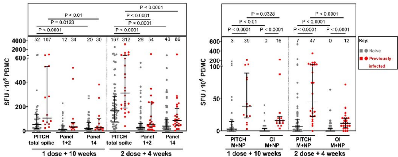
Figure 1 | Comparison of T cell responses to SARS-CoV-2 spike and structural proteins measured by in-house PITCH ELISpot and Oxford Immunotec T-SPOT assay. (A) T cell responses to SARS-CoV-2 spike in naïve and previously-infected healthcare workers reported by three panels: PITCH total spike (S1+S2), Oxford Immunotec Panel 1+2 (diagnostic S1+S2) and Oxford Immunotec Panel 14 (total spike). Friedman test was used for statistical analysis between the 3 panels. (B) T cell responses to SARS-CoV-2 membrane (M) and nucleocapsid (NP) in naïve and previously-infected healthcare workers reported by PITCH ELISpot and Oxford Immunotec (OI) T-SPOT assay. Wilcoxon test was used for statistical analysis between samples matched across both assays, and Mann-Whitney test was used to compare naïve and previously-infected T cell responses within subgroups. (A-B) T cell responses are quantified by spot-forming units per 10 6 peripheral blood mononuclear cells (PBMCs). Healthcare workers received phlebotomy 10 weeks post 1 st dose (1 dose + 10 weeks) and/or 4 weeks post 2 nd dose (2 dose + 4 weeks). All samples are matched across both assays (3 panels for spike and 2 for M+NP T cell responses). At 1 dose + 10 weeks, n=41 for naïve samples and n=14 for previously-infected samples. At 2 dose + 4 weeks, n=75 for naïve samples and n=24 for previously infected samples. Infection status at time of first vaccine, as defined by available PCR and serology data: grey symbols = naïve HCWs and red symbols = HCWs previously infected with SARS-CoV-2. Median T cell responses are stated immediately above each column and marked by a horizontal line on each column, and interquartile range is represented by error bars.
