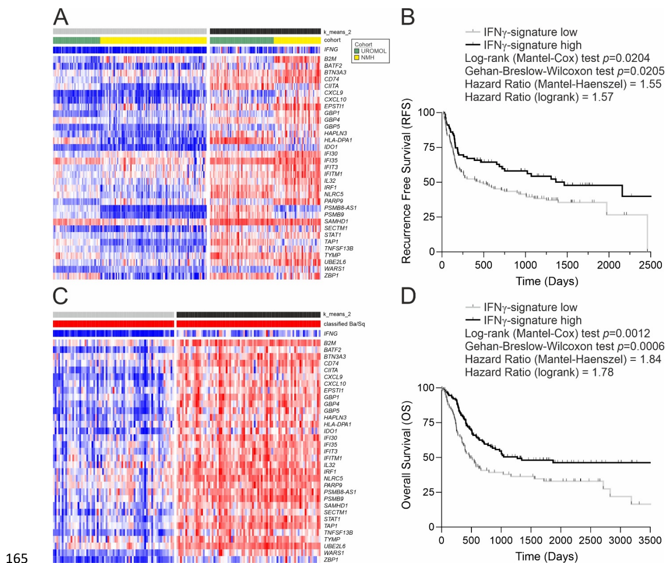
166 Figure 2 – (A) Heatmap and k means clustering based on expression of the IFN \gamma -signature 167 genes in the T1 tumours of UROMOL2021 and Northwestern Memorial Hospital (NMH) 168 cohorts ( n=236 ). The IFN \gamma -signature shows a Spearman rank correlation of 0.66 ( p=4 \times 10^{-31} ) 169 with the IFNG gene in T1 tumours. The full UROMOL2021 cohort is shown as Supplemental 170 Fig. 3; [6]). The separate NMH T1 cohort ( n=99 ; [7]) is shown as Supplemental Fig. 4. (B) 171 Kaplan-Meier analysis of IFN \gamma -signature high and low T1 tumours with survival data from 172 UROMOL2021 and NMH cohorts combined ( n=201 ). The Kaplan-Meier curve is truncated but 173 no events were recorded after the truncation. A Cox proportional hazards regression was 174 also performed using the unit-length scaled IFN \gamma -signature values from T1 tumours which
