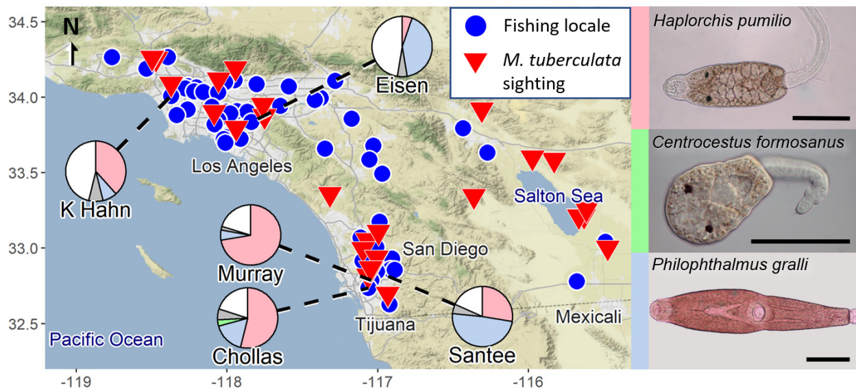
76 Figure 1. The introduced snail, Melanoides tuberculata , and three of its human-pathogenic trematode parasites are 77 widespread throughout southern California. The 25 sites with research-grade M. tuberculata observations from 78 iNaturalist.org (bottom points of red inverted triangles) are well-interspersed among the 55 fishing sites (blue 79 circles) listed by the California Department of Fish & Wildlife at elevations likely suitable for M. tuberculata 80 survival. Surveyed sites are marked by dashed lines leading from pie charts: K Hahn = Kenneth Hahn State 81 Recreation Area (Los Angeles County), Eisen = Eisenhower Park (Orange Co.), Murray = Murray Reservoir (San 82 Diego Co.), Chollas = Chollas Lake Park (San Diego Co.), Santee = Santee Lakes Recreation Preserve (San Diego 83 Co.). Pie charts indicate parasite prevalence at each surveyed site: green = Haplorchis pumilio , gold = 84 Philophthalmus gralli , purple = Centrocestus formosanus , gray = other non-human-pathogenic trematodes, white = 85 uninfected snails. Photographs of heat-stunned, unstained cercariae of each human-pathogenic trematode are coded 86 to their respective color on the pie charts. Scale bar = 100 μm.
