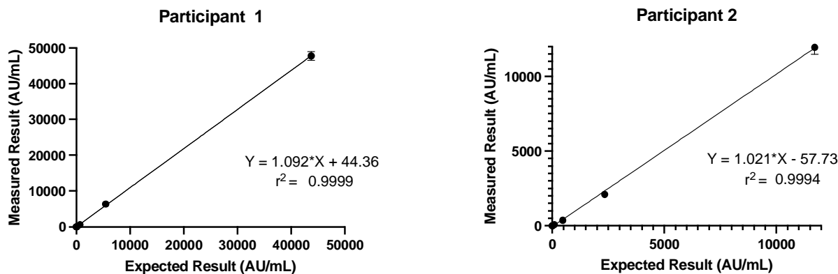
Figure 1 – Linearity of Anti-S IgG
