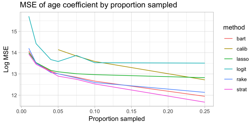
Figure 8: Log MSE as a function of proportion sampled.
