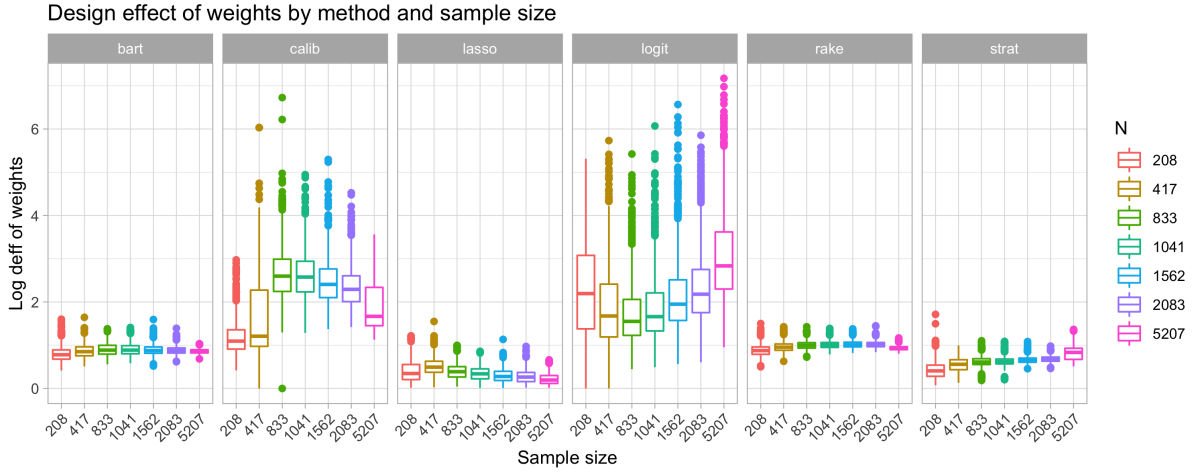
Figure 3: Log design effect by method and sample size in simulation studies
