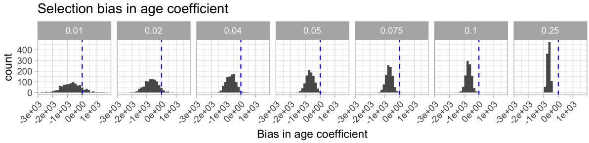
Figure 6: The distribution of estimates of the coefficient for age in a linear regression of total brain volume on age. Regressions were estimated using unadjusted (selection-biased) sample data. The blue lines represent the true population value of the age coefficient.
