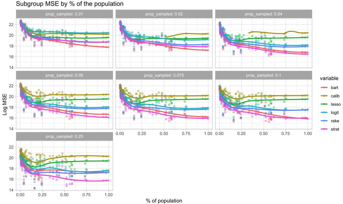
Figure 5: Points represent the log MSE of total brain volume calculated for demographic subgroups, by the true proportion of the population made up by that subgroup. Lines are smoothed estimates of the association between proportion of the population and MSE.
