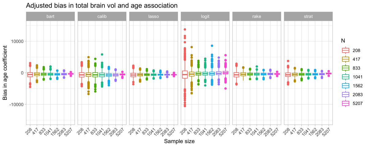
Figure 7: Bias in weighted estimate of age coefficient in regression predicting total brain volume.
