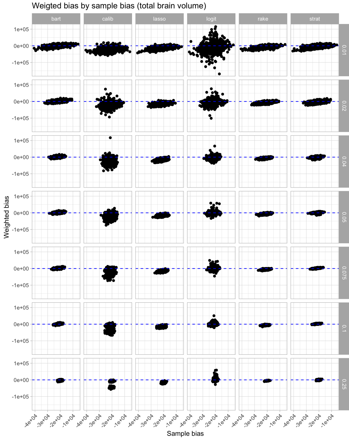
Figure 10: Bias in total brain volume. The x-axis shows the actual selection bias in the sample, the y-axis shows the remaining bias once each adjustment procedure was applied.
