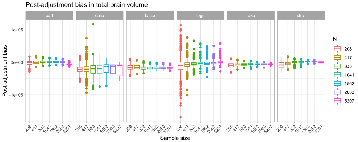
Figure 2: Error by method and sample size in simulation studies
