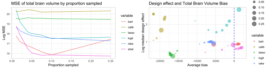
(a) MSE of total brain volume by proportion sampled (b) Log median design effect of weights by average bias in total brain volume
