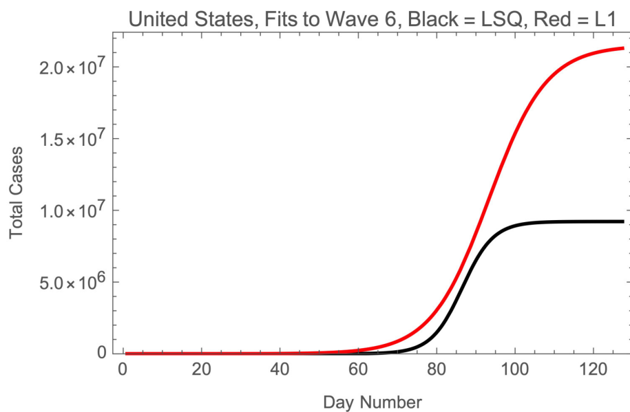
Fig. 13.— Predictions of the logistic model for the total USA cases of COVID-19 in wave 6.
