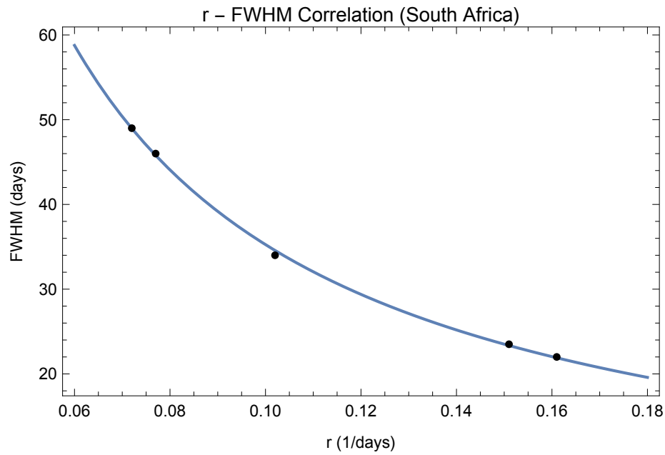
Fig. 6.— Correlation of the growth rate r and the FWHM of each wave for the COVID-19 pandemic in the Republic of South Africa. The curve is Eq. 4. The two pairs of points at the ends are from the LSQ and L1 fits to waves 1 and 4.
