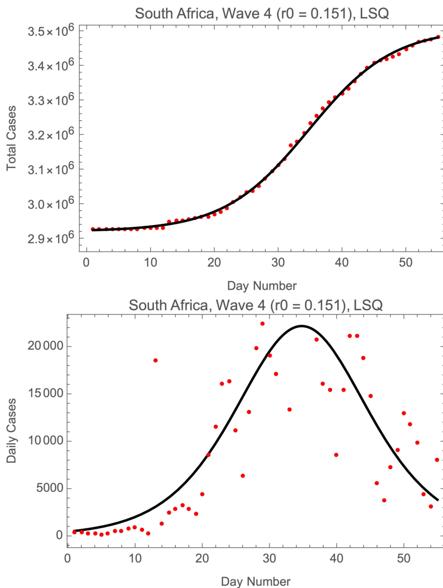
Fig. 5.— Fits of the logistic model to RSA cases of COVID-19 in wave 4. Day 1 is 12 November 2021.
