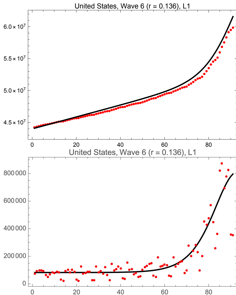
Fig. 10.— L1 fits of the logistic model to total USA cases of COVID-19 in wave 6. Day 1 is 13 October 2021.
