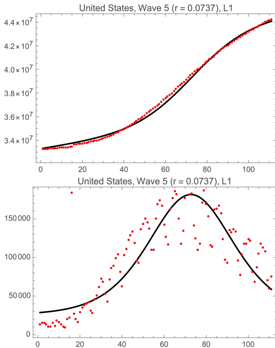
Fig. 9.— L1 fits of the logistic model to USA cases of COVID-19 in wave 5. Day 1 is 25 June 2021.
