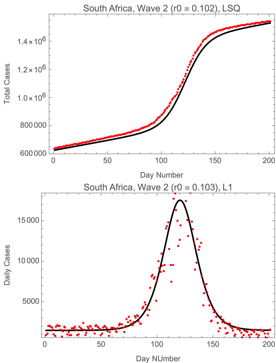
Fig. 4.— Fits of the logistic model to RSA cases of COVID-19 in wave 2. Day 1 is 8 September 2020.
