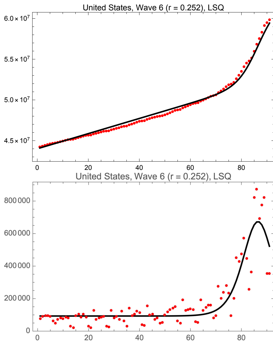
Fig. 11.— LSQ fits of the logistic model to USA cases of COVID-19 in wave 6. Day 1 is 13 October 2021.
