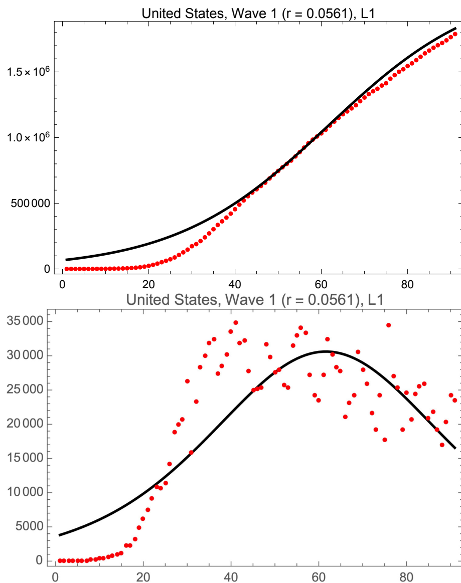
Fig. 7.— L1 fits of the logistic model to USA cases of COVID-19 in wave 1. Day 1 is 20 March 2020.
