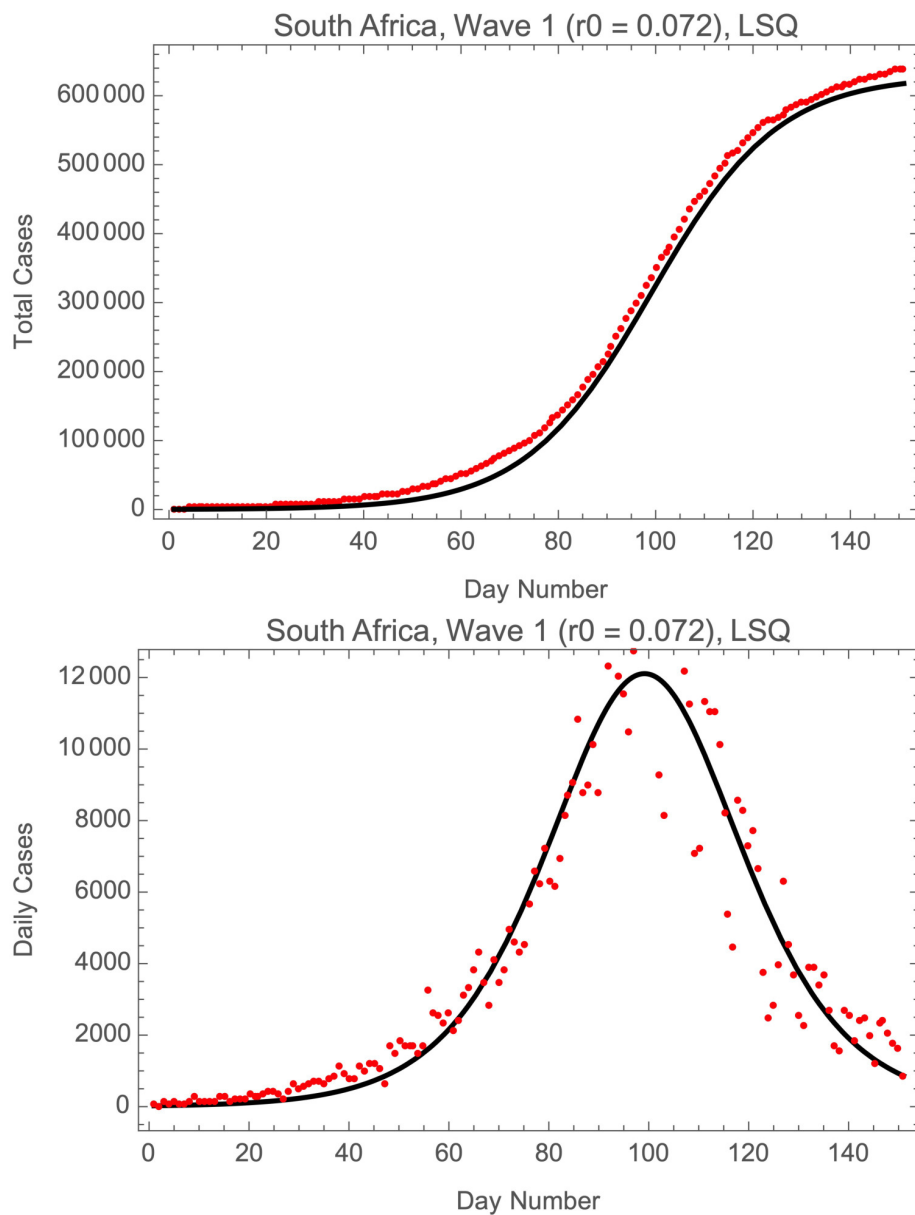
Fig. 3.— Fits of the logistic model to RSA cases of COVID-19 in wave 1. Day 1 is 11 April 2020.
