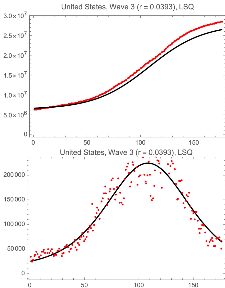
Fig. 8.— LSQ fits of the logistic model to total USA cases of COVID-19 in wave 3. Day 1 is 8 September 2020. is
