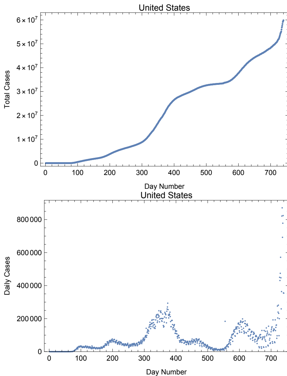
Fig. 1.— Cases data for the entire pandemic for the United States.
