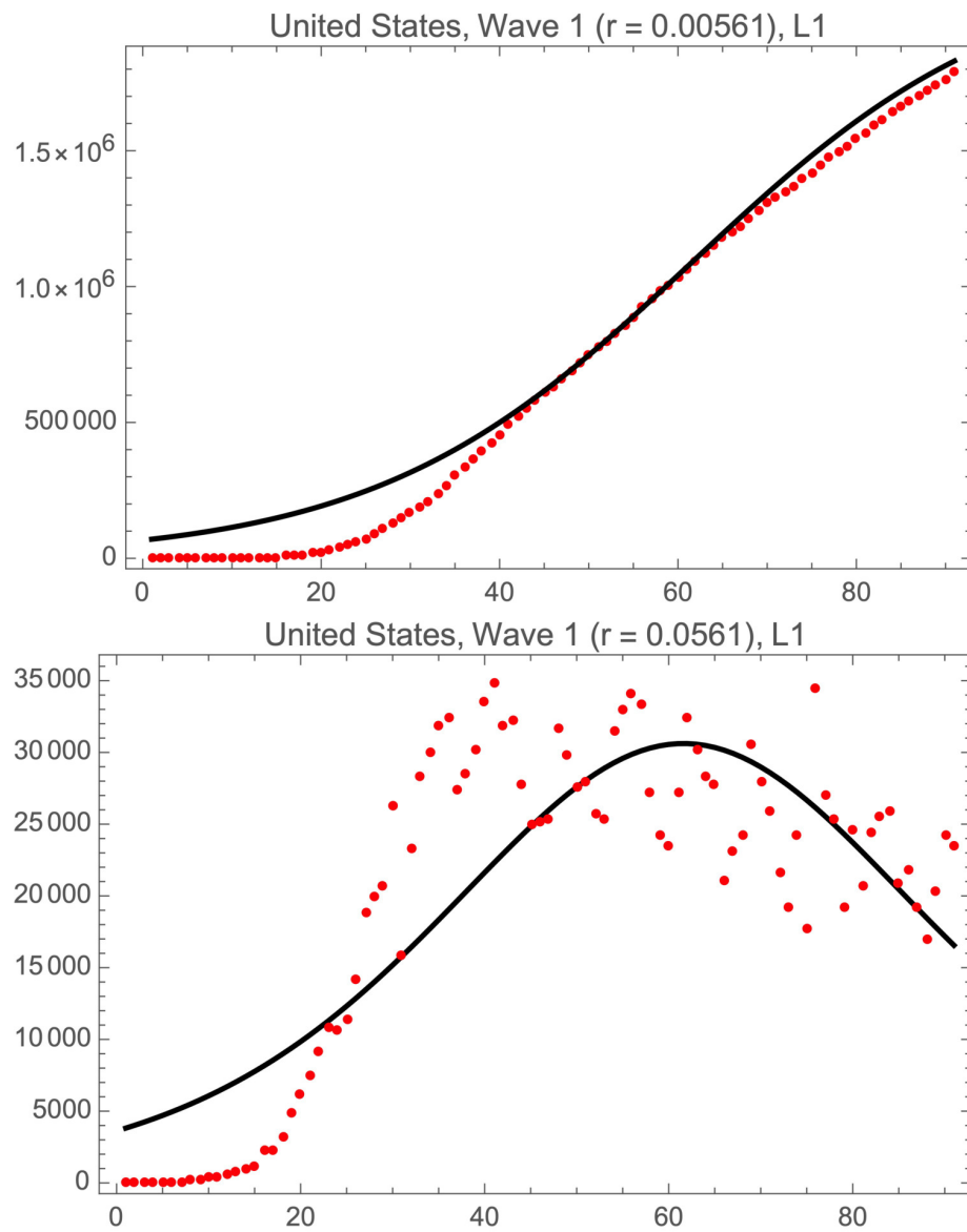
Fig. 7.— L1 fits of the logistic model to USA cases of COVID-19 in wave 1.
