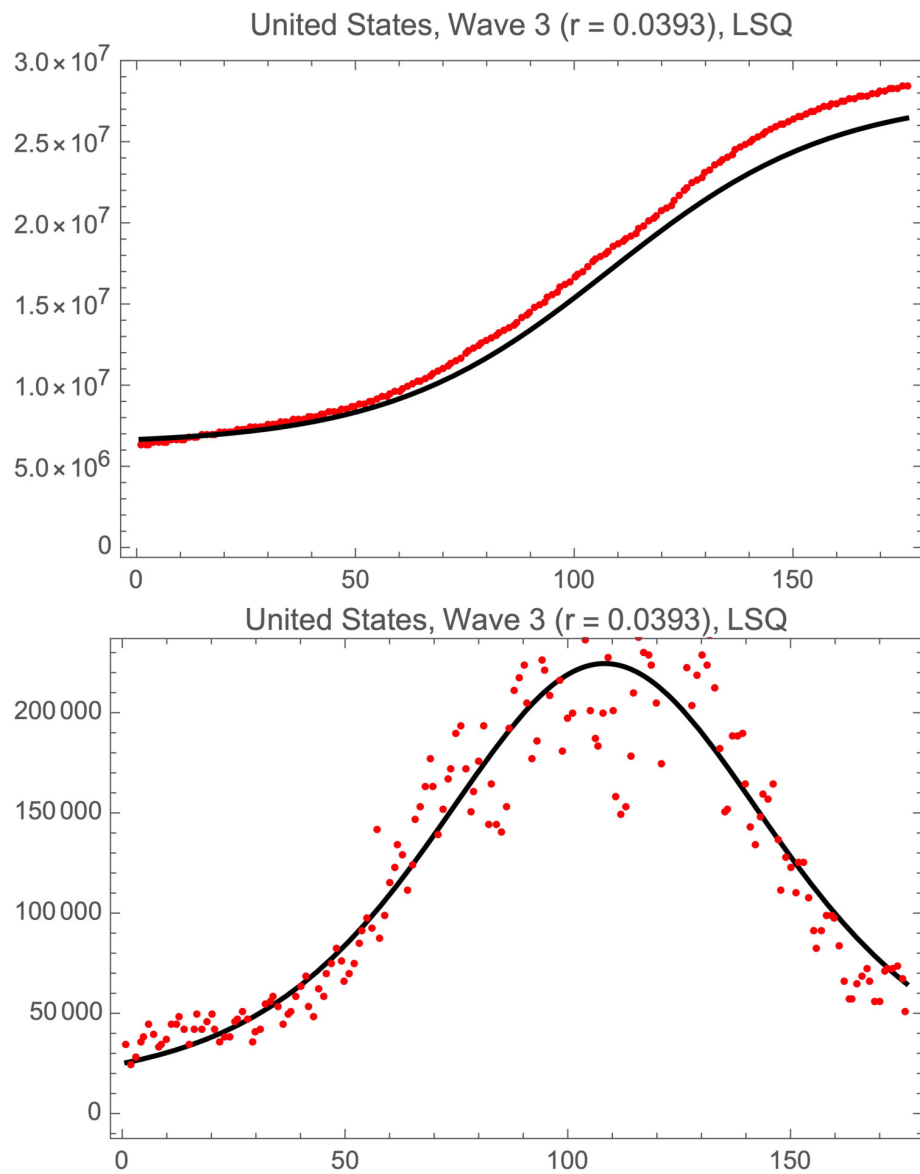
Fig. 8.— LSQ fits of the logistic model to total USA cases of COVID-19 in wave 3.
