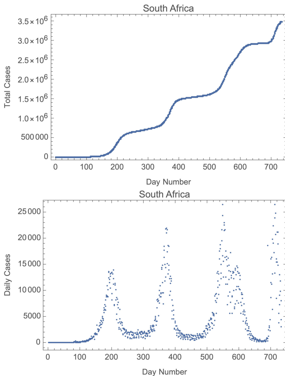
Fig. 2.— Cases data for the entire pandemic for the Republic of South Africa..
