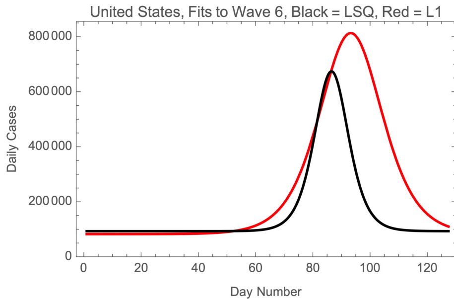
Fig. 14.— Predictions of the logistic model for the daily USA cases of COVID-19 in wave 6.
