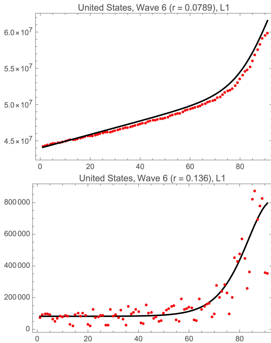
Fig. 10.— L1 fits of the logistic model to total USA cases of COVID-19 in wave 6
