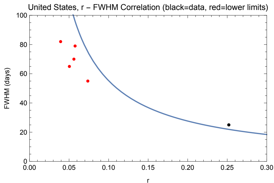
Fig. 12.— Correlation of the growth rate r and the FWHM of each wave for the COVID-19 pandemic in the United states. The curve is Eq. 4. The black point is the measurement for wave 6 using the LSQ solution, the red points are lower limits for the widths of the other waves.
