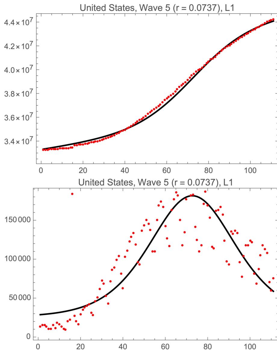
Fig. 9.— L1 fits of the logistic model to USA cases of COVID-19 in wave 5
