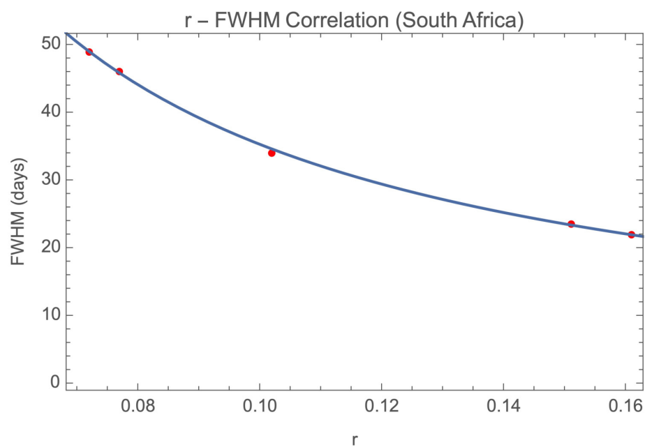
Fig. 6.— Correlation of the growth rate r and the FWHM of each wave for the COVID-19 pandemic in the Republic of South Africa. The curve is Eq. 4. The two pairs of points at the ends are from the LSQ and L1 fits to waves 1 and 4.
