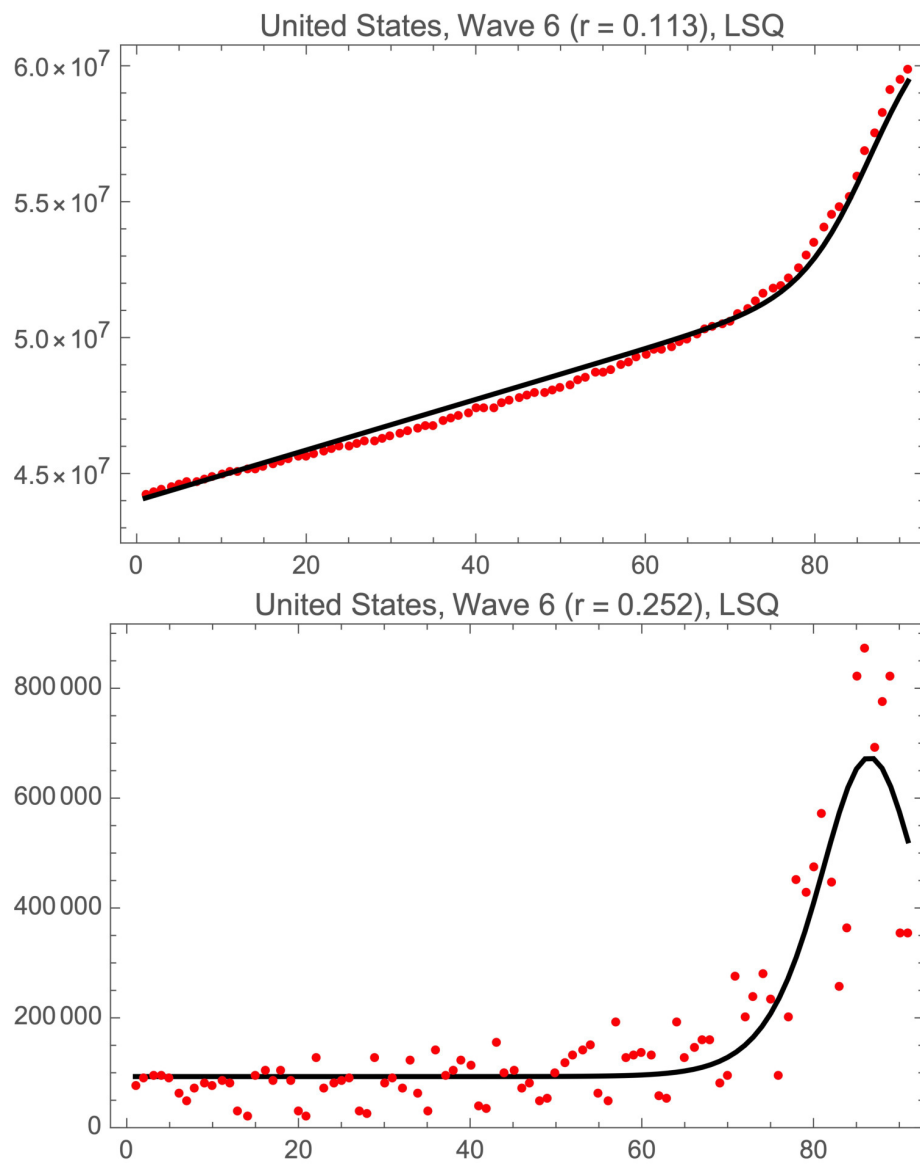
Fig. 11.— LSQ fits of the logistic model to USA cases of COVID-19 in wave 6
