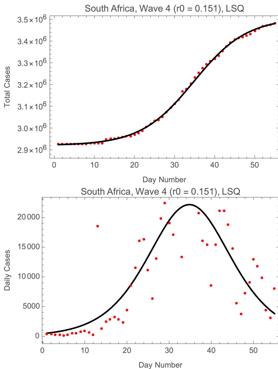
Fig. 5.— Fits of the logistic model to RSA cases of COVID-19 in wave 4.
