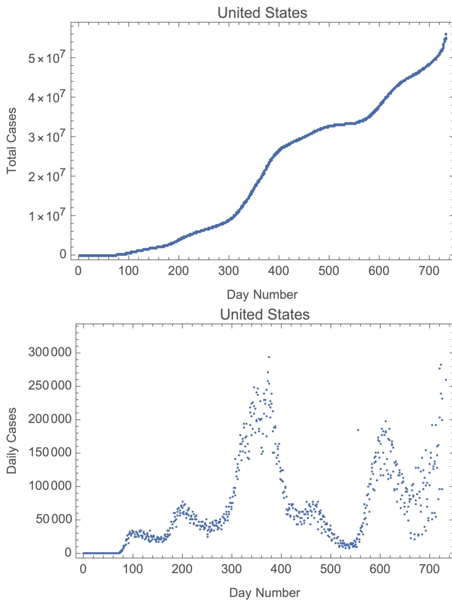
Fig. 1.— Cases data for the entire pandemic for the United States.
