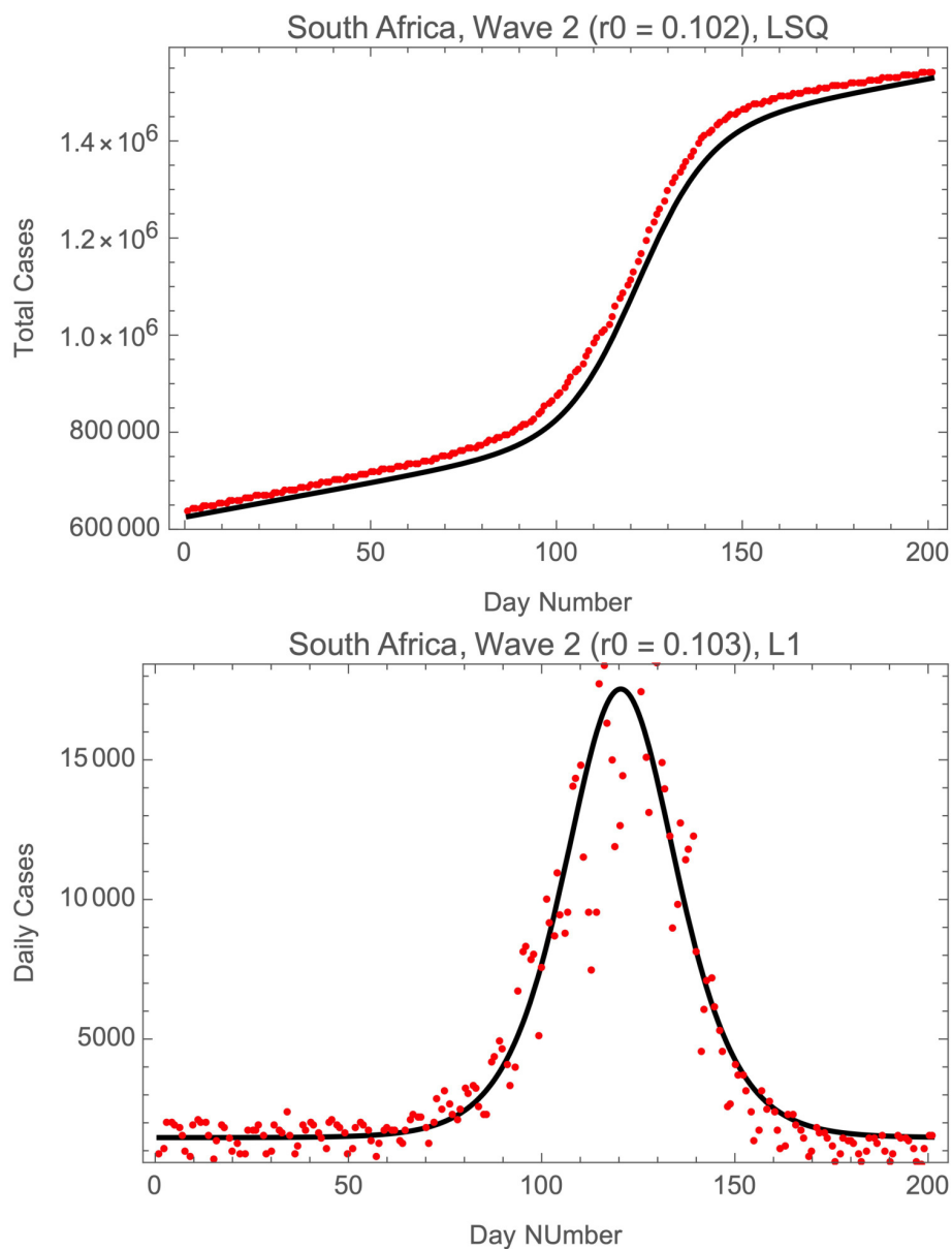
Fig. 4.— Fits of the logistic model to RSA cases of COVID-19 in wave 2.
