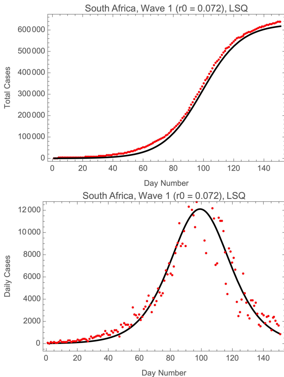
Fig. 3.— Fits of the logistic model to RSA cases of COVID-19 in wave 1.
