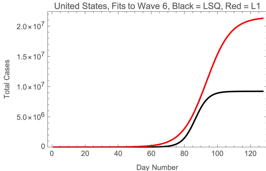
Fig. 13.— Predictions of the logistic model for the total USA cases of COVID-19 in wave 6.
