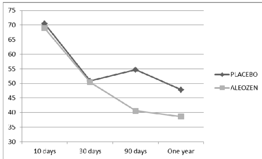
Figure 3: Evolution of the mean of CAPS-5 between Aleozen and Placebo groups over time
