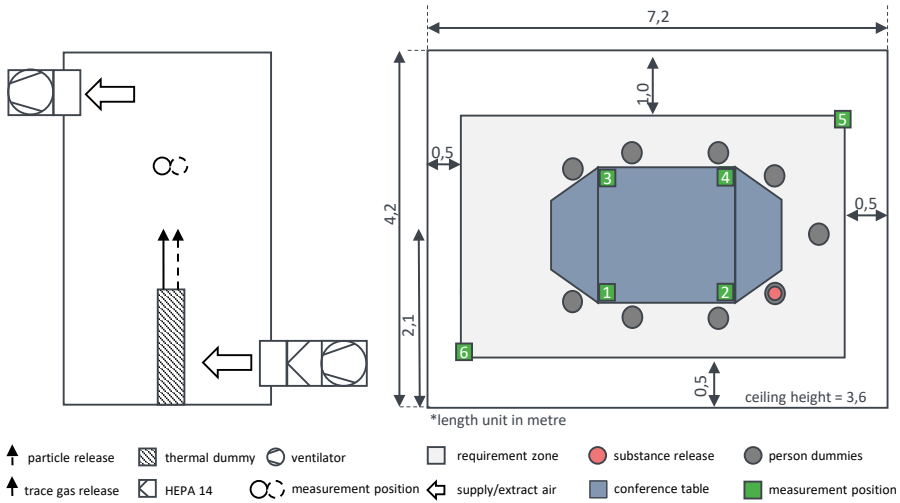
Fig. 3 set up to compare both methods (left) and top view of the conference room (right)
