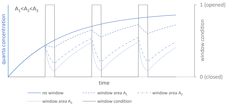
Fig. 2 quanta concentration course for periodic ventilation depending on different opened window areas
