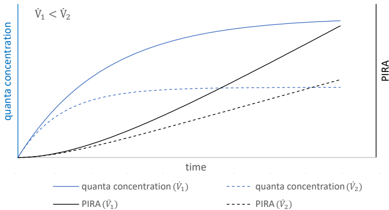
Fig. 1 quanta concentration and PIRA course for different device volume flows
