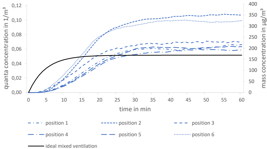
Fig. 7 theoretical (ideal mixed air) and measured quanta concentration (left axis) and their related mass concentration (right axis) of six positions in a two-person office
