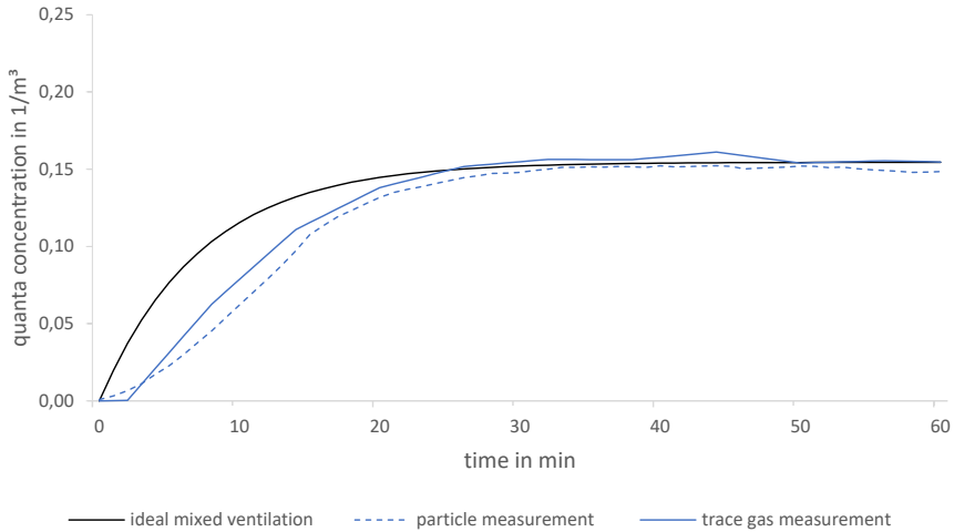
Fig. 4 comparison between particle and trace gas measurement as a function of quanta concentration over time exemplified in a conference room (position 3)
