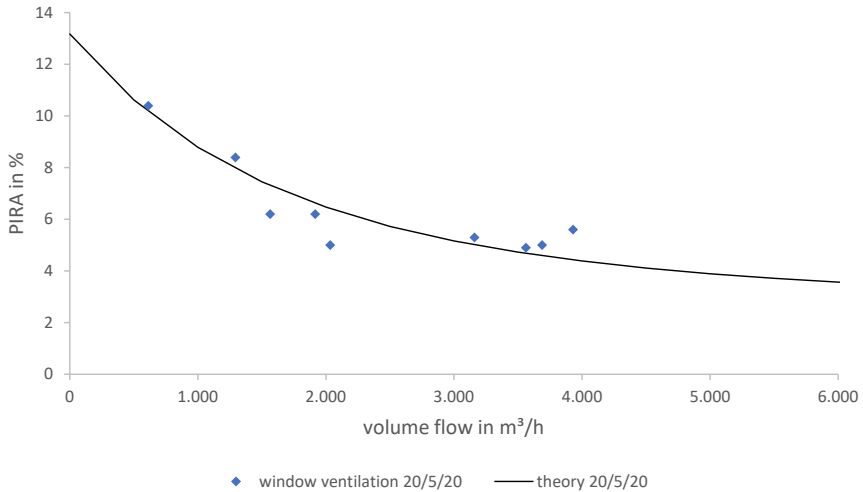
Fig. 9 infection risk over occurring volume flow for periodic window ventilation
