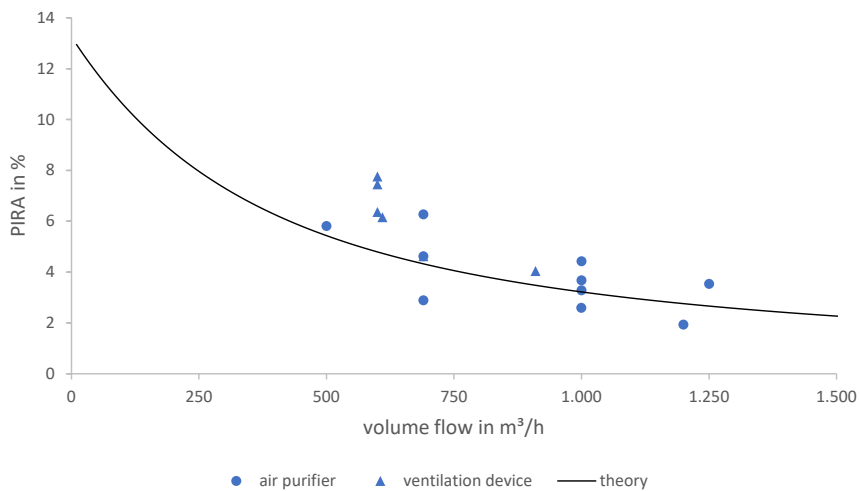
Fig. 10 infection risk over continuously operating ventilation systems or air purifiers
