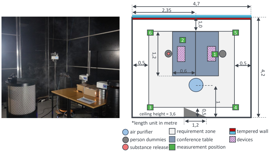
Fig. 6 photo (left) and the top view (right) of the experimental set up of a two person office with air purifiers in an air visualisation laboratory
