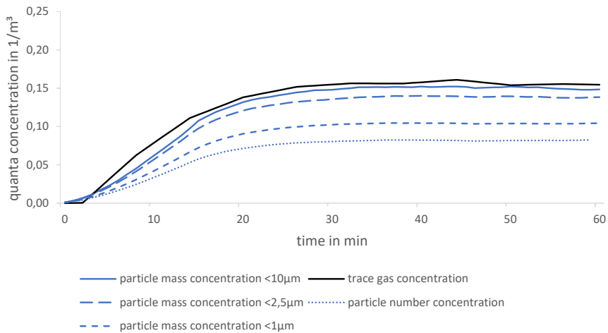
Fig. 11 comparison of quanta concentrations based on particle mass, particle number and trace gas concentrations in a conference room
