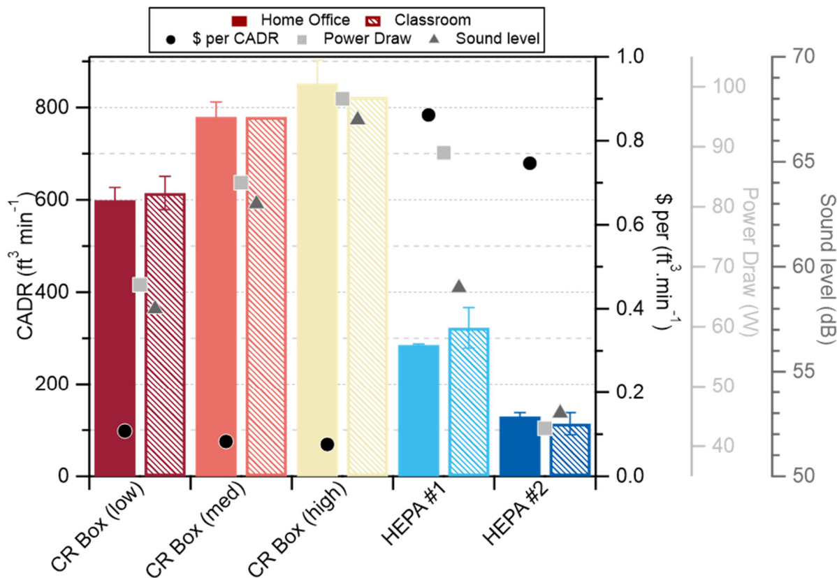
Figure 2. (left axis) The number-weighted clean air delivery rate for the various air filters (left axis, bars) as measured in the home office (left hash marks) and classroom (right hash marks). (right axis) The price normalized CADR (black circles), sound level (dark gray triangles), and power (light gray squares).
