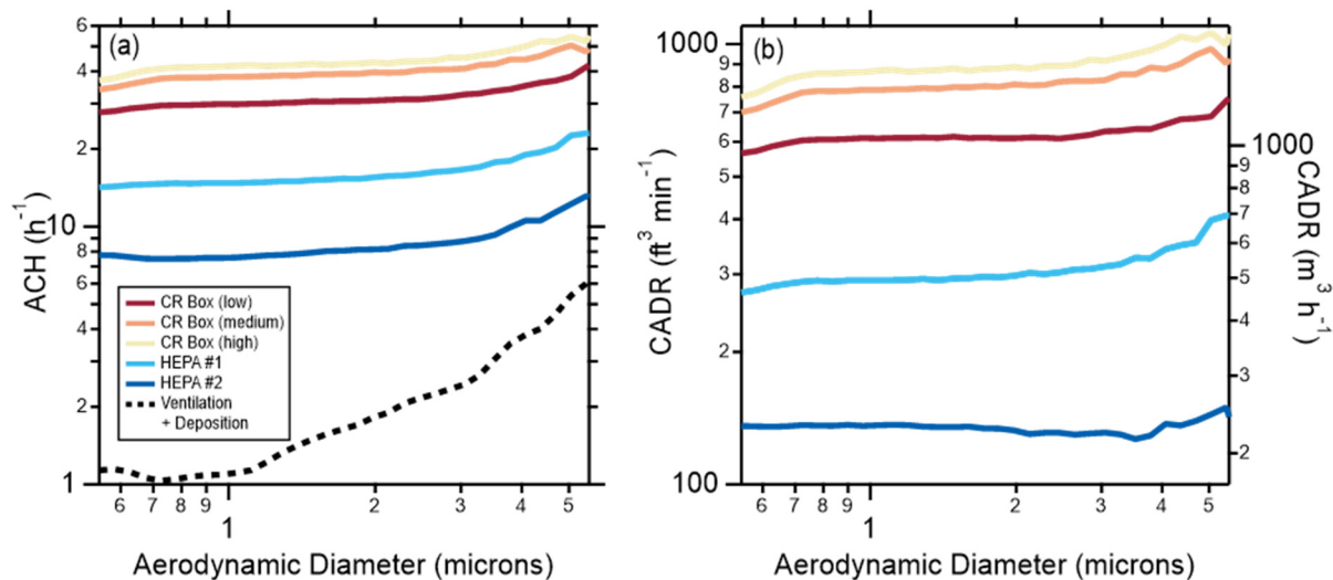
Figure 3. (a) Size-dependent air changes per hour with the various air filters operating (solid lines) and for the natural room ventilation + particle deposition alone (dashed line), as measured in the home office. (b) The corresponding clean air delivery rates for the various air filters. Results for the classroom are similar (not shown).
