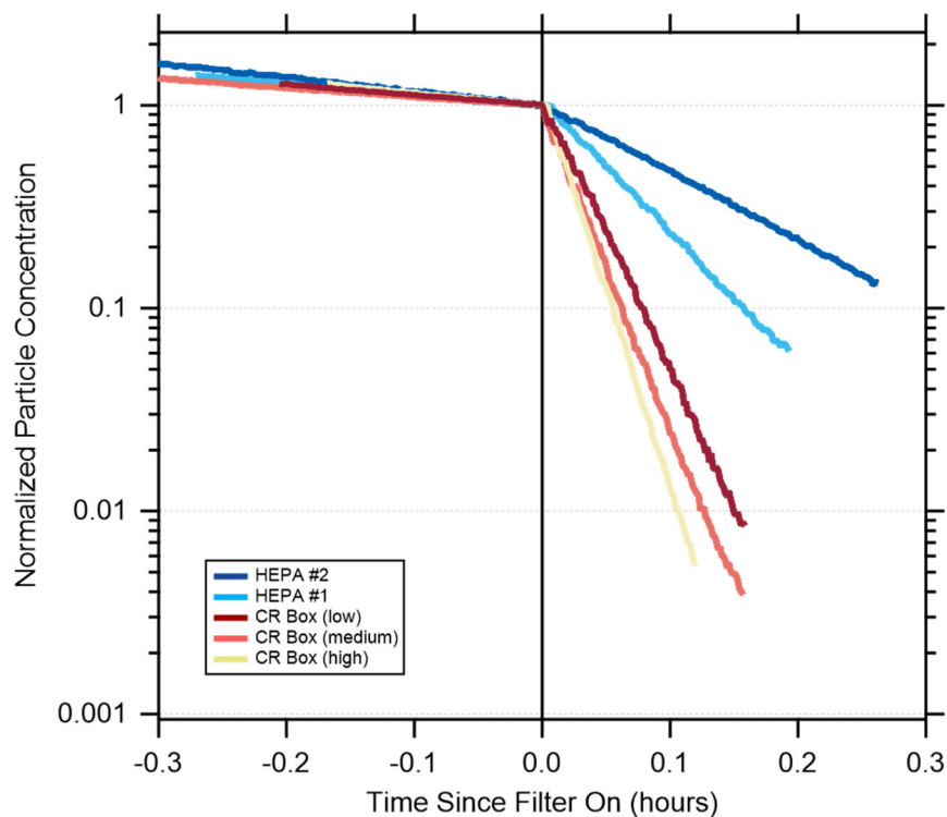
Figure 1. Example particle number decays measured in the home office for the natural ventilation + particle deposition (at t < 0 ) and with the air filters on ( t > 0 ). Particle concentrations have been normalized to unity at t = 0 .
