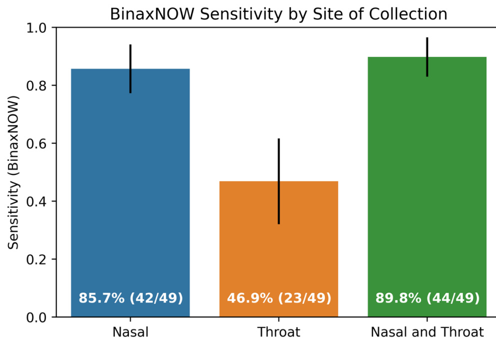
Figure 2. Sensitivity of BinaxNOW tests by site of collection based on samples collected on January 14 (N=115). Sensitivity is calculated using either nasal or throat RT-PCR as the referent for samples with Ct less than 30. Bar height indicates the calculated sensitivity for the indicated site of collection; error bars indicate the 95th percentile confidence interval as calculated using the Clopper-Pearson method. “Nasal and throat” indicates a BinaxNOW positive result in either the nasal or throat or both samples. The calculated sensitivity, expressed both as a percent and a fraction, is overlaid on the corresponding bar. Abbreviations: COVID-19, coronavirus disease 2019; Ct, cycle threshold; RT-PCR, reverse transcription polymerase chain reaction.
