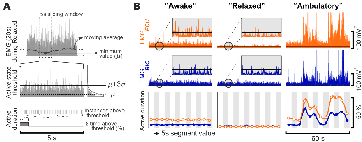
404 Figure 1. Proposed time-based sEMG measure: Active duration. (A) Conditioned sEMG is 405 examined with a moving average window (e.g., 5 s) to find the minimum across all recordings 406 (top), from which a threshold of active state was defined (middle). Active duration is calculated 407 for each segment as the percent of time amplitude was above the threshold (bottom). (B) Time 408 trace of conditioned sEMG and calculated active duration (bottom) over 60 s from a representative 409 participant with stroke during normal Awake , completely Relaxed , and functional Ambulatory 410 states.
