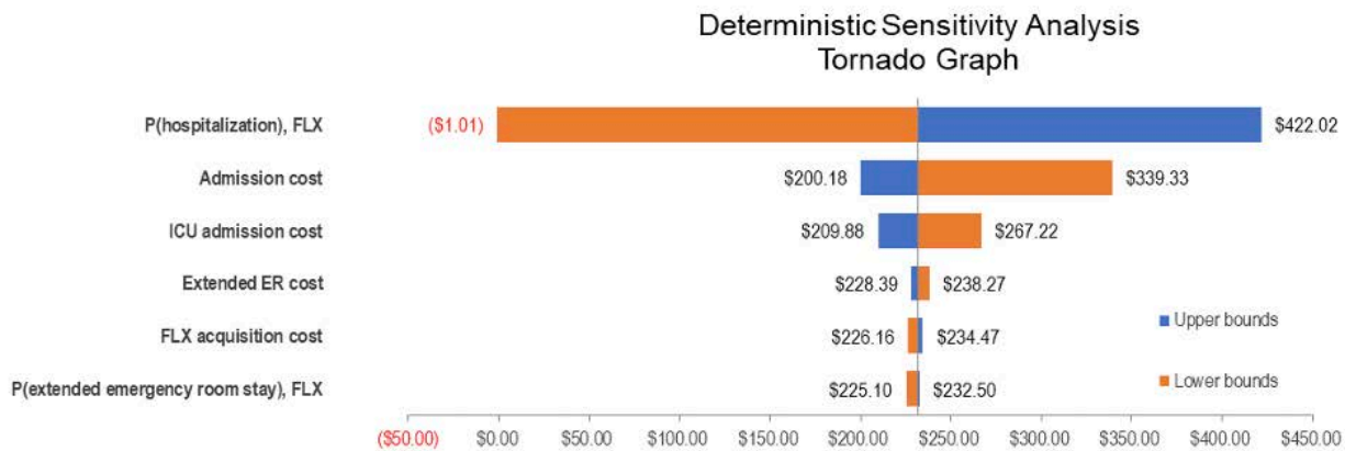
Figure 2. Tornado diagram for one-way sensitivity analyses
