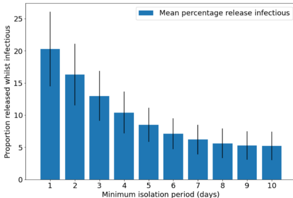
Figure 1: Sensitivity of the model to different testing regimes. People will not necessarily be released on the first day possible but when they have two consecutive negative LFD tests, or when they reach 10 days. We are measuring the cumulative effects over all releases over all the days
