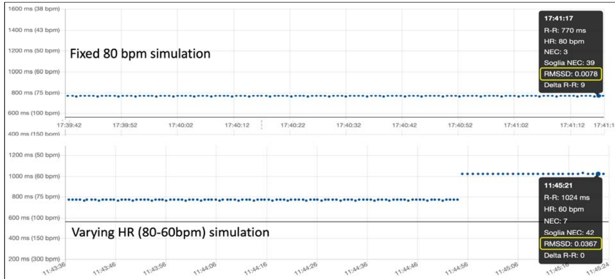
Figure 2. While the physiological heart rate variability usually corresponds to a RMSSD index around 0.025 in adults in the sitting position, the simulation with a fixed heart rate (Top) does not account for physiological RR variability (RMSSD 0.0078), while varying heart rate between 80bpm and 60 bpm in the simulation brings the RMSSD index back to the order of magnitude of physiological values (RMSSD 0.0367) (Bottom).
