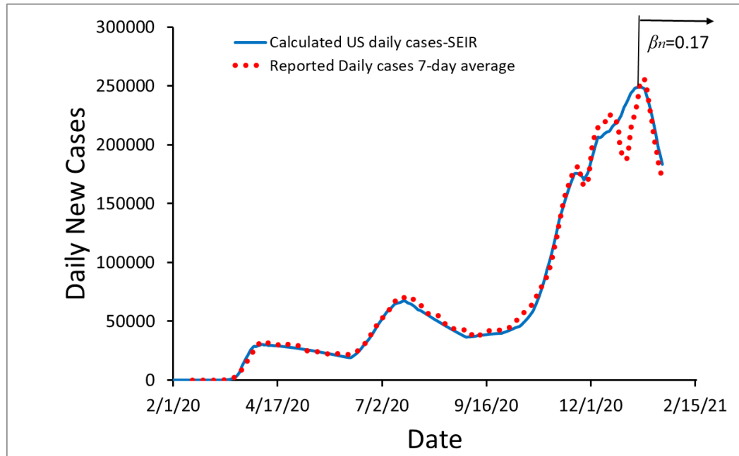
Figure 4. The number of daily new COVID-19 cases reported from 2/15/2020 to 1/22/2021 in the United States (red dots) and the number of daily new COVID-19 cases calculated from the new SEIR model in the same period (blue line).
