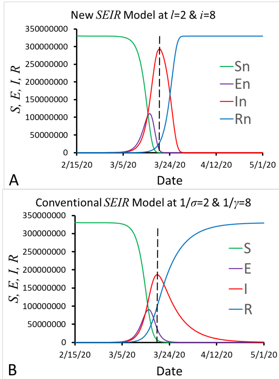
Figure 2. Comparison of S , E , I and R calculated from the new SEIR model (A) with S , E , I and R calculated from the conventional SEIR model (B) assuming that the latent period l=1/\sigma=2 days and the infectious period i=1/\gamma=8 days.
