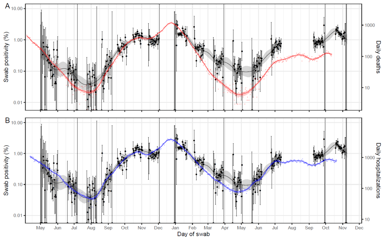
Figure 3. (A) comparison of daily deaths and hospitalisations to swab-positivity as measured by REACT-1. Daily swab-positivity for all 15 rounds of the REACT-1 study (black points with 95% confidence intervals, left-hand y-axis) with P-spline estimates for swab-positivity (solid black line, shaded area is 95% credible interval). Daily deaths in England (red points, right-hand y-axis) and P-spline model estimates for expected daily deaths in England (solid red line, shaded area is 95% credible interval, right-hand y-axis). Daily deaths have been shifted by 25 (25, 26) days backwards in time along the x-axis. The daily deaths (right-hand) y-axis has been scaled using the best-fit population adjusted scaling parameter 0.060 (0.058, 0.062). (B) Daily hospitalisations in England (blue points, right-hand y-axis) and P-spline model estimates for expected daily hospitalisations in England (solid blue line, shaded area is 95% credible interval, right-hand y-axis). Daily hospitalisations have been shifted by 19 (18, 20) days backwards in time along the x-axis. The daily hospitalisations (right-hand) y-axis has been scaled using the best-fit population adjusted scaling parameter 0.238 (0.230, 0.246).
