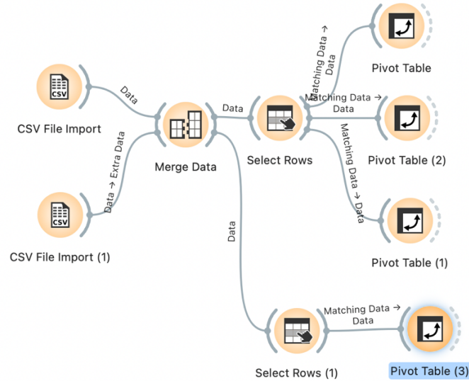
Figure 3 Algorithm for genomic analysis and monitoring of VOC ij Delta = [Delta (WHO label)], [G / 478K.V1 (GISAID clade)], [B.1.617.2 + AY.x (Pango lineage)] del (SARS -CoV-2) COVID-19 in Mexico
