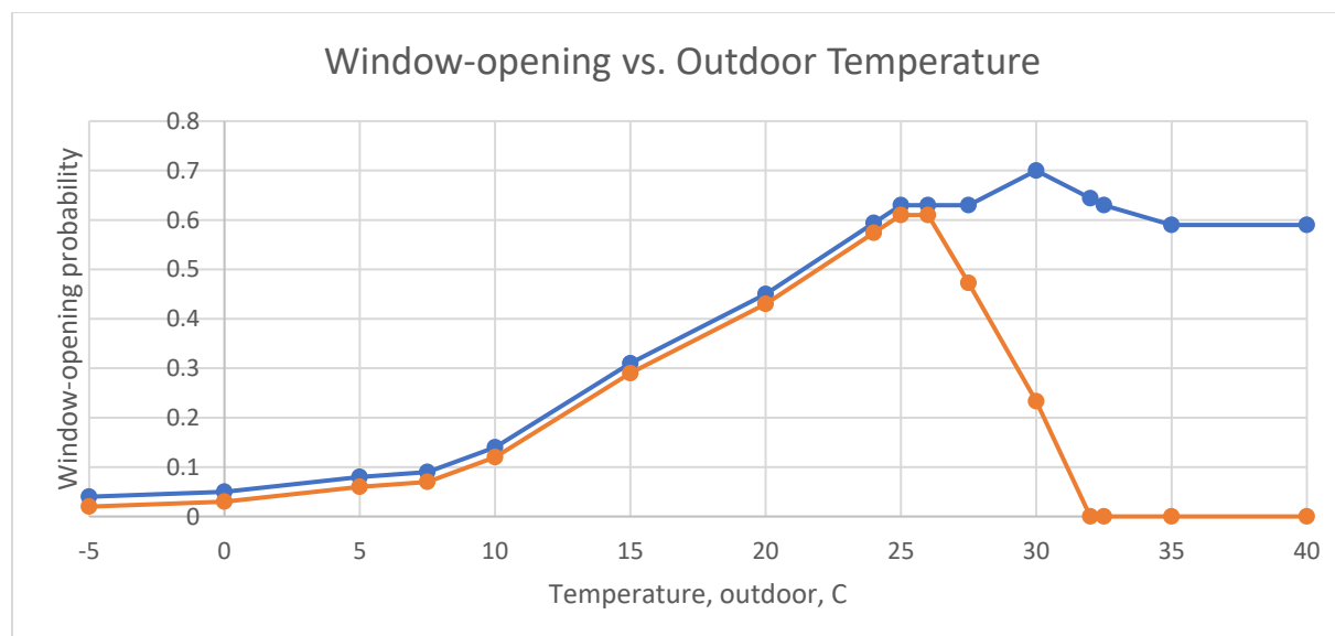
Figure 6. The probability of window-opening as a function of outdoor temperature, without air conditioning (blue line), and in households with air conditioning (orange line), based on the figures from the literature in Table 3.
