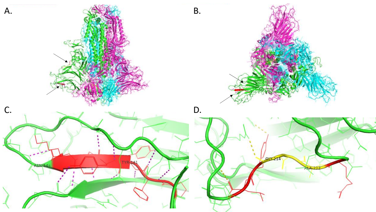
Figure 4. Three-dimensional structure of the SARS-CoV-2 spike glycoprotein illustrating the location of the A.2.5 INDELS 141-143 deletion and 215AGY insertion in the N-terminal domain. The structure is colored by domain and shown from the front view (A) and rotated to view the receptor binding site (B). The arrows point to the LGV deletion at Spike 141 and AGY insertion at 215, colored red to highlight their location in the NTD. The structural impact of the Spike 141-143 deletion and 215 insertion are shown in (C) and (D), respectively. Three flanking amino acids of the INDELS are colored in red, and insertions are colored yellow.
