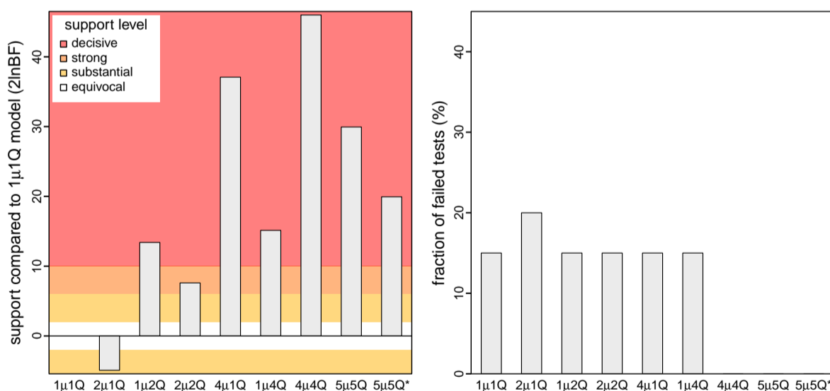
Fig. 5. An interval-specific model provides the best relative and absolute fit to our SARS-CoV-2 dataset. We assessed the relative and absolute fit of nine candidate discrete-geographic phylodynamic models to our study dataset (comprised of all publicly available SARS-CoV-2 genomes from the early phase of the COVID-19 pandemic). Left) We compared the relative fit of each candidate model to the constant-rate ( 1\mu1Q ) phylodynamic model using Bayes factors, which indicate that the 4\mu4Q interval-specific model outcompetes both less complex and more complex models. Right) We performed posterior-predictive simulation for each candidate model using 20 summary statistics, plotting the fraction of those summary statistics indicating that a given candidate model was inadequate. Our results indicate that three candidate models ( 4\mu4Q , 5\mu5Q , and 5\mu5Q^* ) provide an adequate fit to our SARS-CoV-2 dataset. The simplest of these adequate models ( 4\mu4Q ) also provides the best relative fit. Collectively, these results identify the 4\mu4Q model as the clear choice for phylodynamic analyses of our study dataset.
