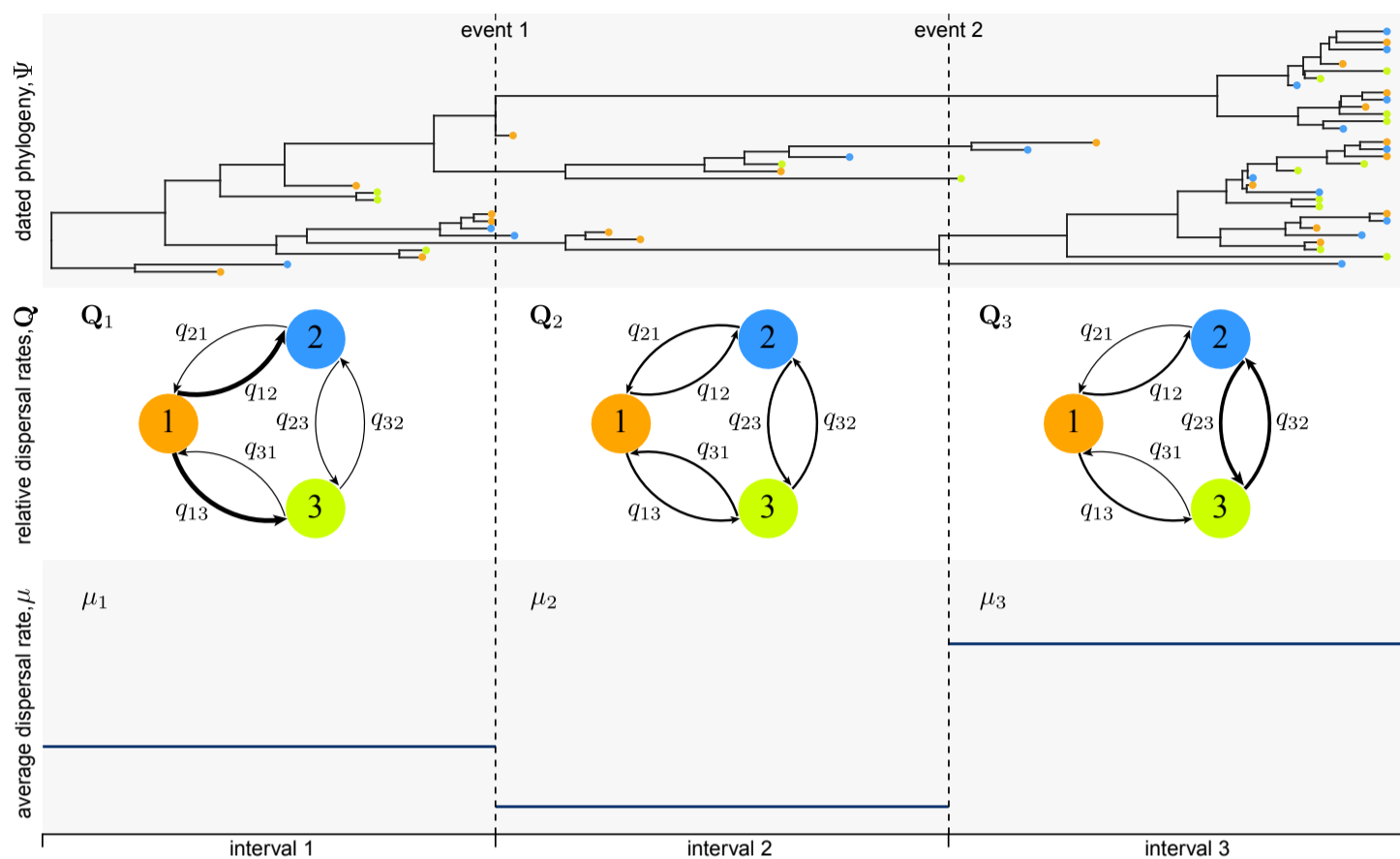
Fig. 1. Interval-specific discrete-geographic phylodynamic models accommodate variation in the process of viral dispersal. Phylodynamic models include two main components: a phylogenetic model that specifies the relationships and divergence times of the sampled viruses, \Psi (top panel), and a biogeographic model that describes the history of viral dispersal among a set of discrete-geographic areas—here, areas 1 (orange), 2 (blue), and 3 (green)—from the root to the tips of the dated viral tree. Parameters of the biogeographic model include an instantaneous-rate matrix, \mathbf{Q} , that specifies relative rates of viral dispersal between each pair of areas (here, each element of the matrix, q_{ij} , is represented as an arrow that indicates the direction and relative dispersal rate from area i to area j ; middle panel), and a parameter that specifies the average rate of viral dispersal between all areas, \mu (lower panel). Although most phylodynamic studies assume that the process of viral dispersal is constant through time, disease outbreaks are typically punctuated by events that impact the average and/or relative rates of viral dispersal among areas. Here, for example, the history involves two events ( e.g. , mitigation measures) that define three intervals, where both \mathbf{Q} and \mu are impacted by each of these events, such that the interval-specific parameters are (\mathbf{Q}_1, \mathbf{Q}_2, \mathbf{Q}_3) and (\mu_1, \mu_2, \mu_3) . Our framework allows investigators to specify discrete-geographic phylodynamic models with two or more intervals, where each interval has independent relative and/or average dispersal rates, which are then estimated from the data.
