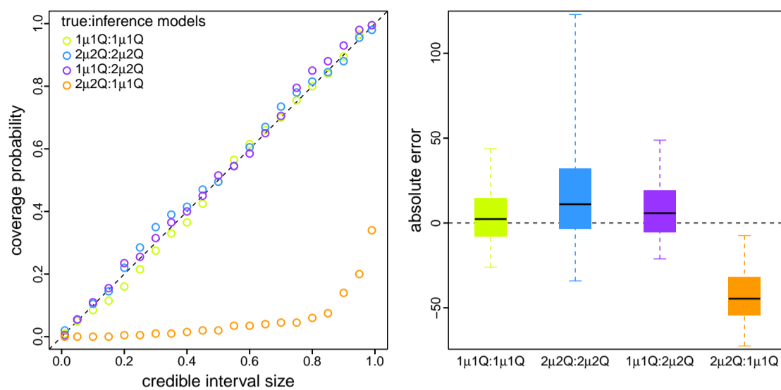
Fig. 3. Simulation demonstrates that reliable inference of viral dispersal history requires a correctly specified discrete-geographic phylodynamic model. We simulated 200 geographic datasets under each of two models: one that assumed a constant \mu and Q ( 1\mu1Q ), and one that allowed \mu and Q to vary over two intervals ( 2\mu2Q ). For each simulated dataset, we separately inferred the total number of dispersal events under each model, resulting in four true:inference model combinations ( 1\mu1Q:1\mu1Q , 2\mu2Q:2\mu2Q , 1\mu1Q:2\mu2Q , and 2\mu2Q:1\mu1Q ). Left) For each combination of true and inference model, we computed the coverage probability (the frequency with which the true number of dispersal events was contained in the corresponding X\% credible interval; y-axis) as a function of the size of the credible interval (x-axis). When the model is true, we expect the coverage probability to be equal to the size of the credible interval (Cook et al., 2006). As expected, coverage probabilities fall along the one-to-one line when the model is correctly specified (green and blue). Moreover, coverage probabilities are also appropriate when the inference model is overspecified ( i.e. , the inference model includes interval-specific parameters not included in the true model; purple). However, coverage probabilities are extremely unreliable when the inference model is underspecified ( i.e. , the inference model excludes interval-specific parameters of the true model; orange). Right) For each true:inference model combination, we summarized the absolute error (estimated minus true number of dispersal events) as boxplots (median [horizontal bar], 50% probability interval [boxes], and 95% probability interval [whiskers]). Again, when the model is underspecified (orange) inferences are strongly biased compared to those under the correctly specified (green and blue) and overspecified (purple) models.
