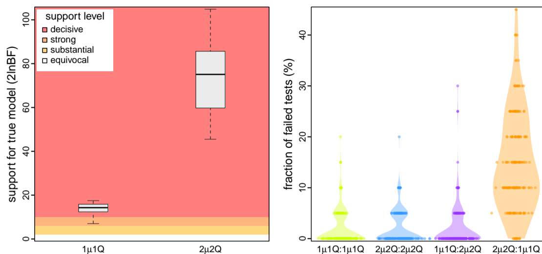
Fig. 4. Simulation demonstrates our ability to accurately identify a correctly specified discrete-geographic phylodynamic model. We assessed the relative and absolute fit of alternative models to the simulated datasets described in Fig. 3. Left) For each simulated dataset, we compared the relative fit of the true and alternative models using Bayes factors. The boxplots summarize Bayes factors for datasets simulated under the constant-rate ( 1\mu1Q , left) and interval-specific ( 2\mu2Q , right) models, which demonstrate that we are able to decisively identify the true phylodynamic model. Right) For each combination of true:inference model, we assessed absolute model fit using posterior-predictive simulation with a set of 20 summary statistics. Each dot represents the fraction of those 20 summary statistics for which the corresponding inference model provides an inadequate fit to a single simulated dataset. The violin plots summarize the distribution of these values for all datasets under each true:inference model combination. As expected, the true model is overwhelmingly inferred to be adequate (green and blue). Encouragingly, model overspecification appears to have a negligible impact on model adequacy (purple). By contrast, an underspecified model severely impacts model adequacy (orange).
