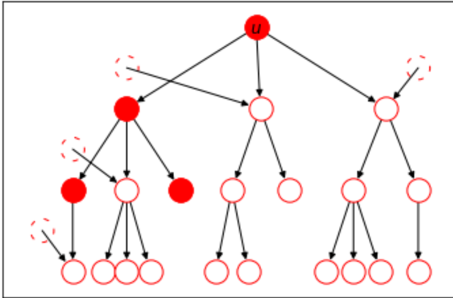
Figure 9: A schematic showing the descendants of u with filled circles showing those whose infections would be averted if u isolates after infection. Dashed hollow circles denotes infected individuals that are not descendants of u who provide additional transmission paths to some descendants of u . Hollow circles with solid boundaries denote the individuals whose infection is overdetermined.
