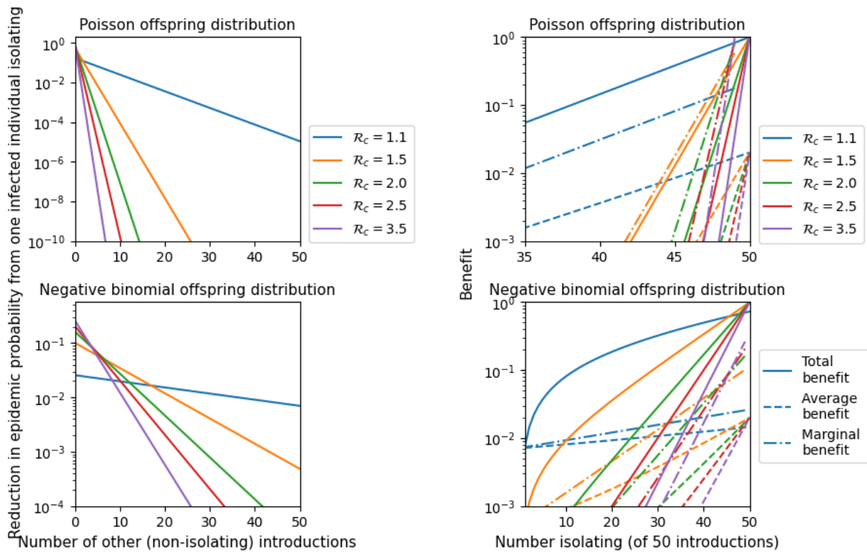
Figure 2 The benefit measured as the reduction in probability of an epidemic. We use a Poisson offspring distribution and a negative binomial offspring distribution with dispersion 0.16. We assume that L infected individuals enter the population of whom M isolate. Left (note different vertical scales): The reduction in epidemic probability if M = 1 (only one isolates) as a function of the number ( L - 1 ) who do not isolate. Due to overdetermination, this decreases as L increases. Right (note different horizontal scales): The reduction in probability if M isolate out of L = 50 introduced cases. This shows the total reduction in epidemic probability (solid line), the reduction averaged across the M isolating individuals (dashed line), and the marginal benefit of the M + 1^{\text{th}} isolating individual, (i.e., the change in probability from the next individual isolating) (dash-dot line). Each additional individual who isolates increases the average impact of all isolating individuals, as a consequence of declining overdetermination.
