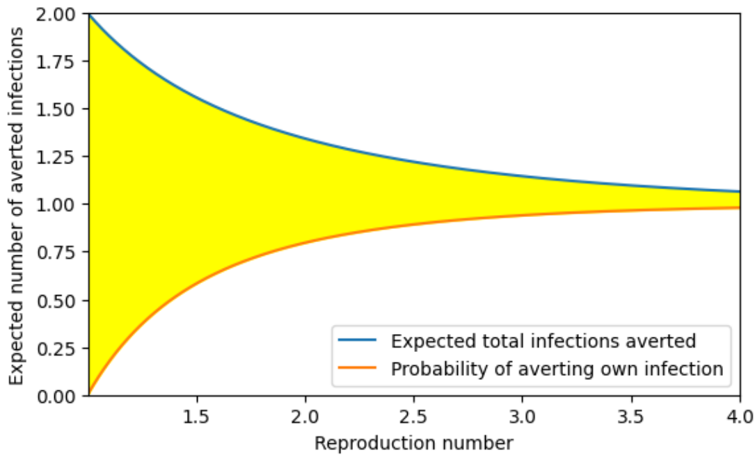
Figure 6: The expected total number of infections averted by an individual taking sufficient action (such as a vaccine or prophylactic medication) to prevent her own infection (top blue curve) for R_c > 1 . This is partly from the probability that she prevents her own infection [bottom orange curve, equal to A(R_c) ] -- note that the probability of averting her own infected equals the expected number of her own infections averted. The other part of the total benefit is because some of her descendants end up uninfected, shown in the difference between the two curves (shaded yellow) F(R_c)A(R_c) .
