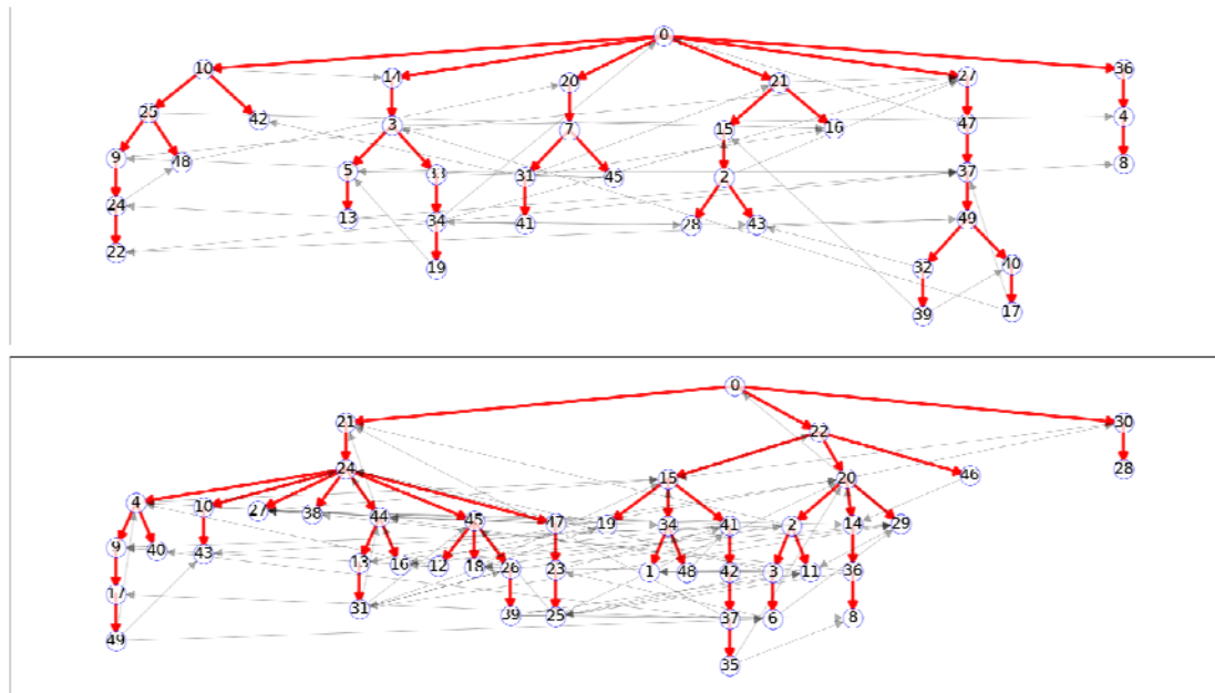
Figure 8 Two sample outbreaks with R_c = 1.5 (top) and R_c = 2.5 (bottom), each starting from a single infection in a population of 50 individuals. Only the eventually infected nodes are shown. The red lines denote successful transmissions while the gray lines denote transmissions from an infectious individual to one who had already been infected. Note that given the transmissions in the R_c = 1.5 case, had individual 36 (second row on right) been the initial infection, only individuals 36, 4, and 8 would have been infected. Additionally, had individual 49 (fifth row on right) isolated after infection (or been effectively protected from infection), this would have prevented the infections of 32, 39, 40, and 17. In the R_c = 2.5 case, there are many more (potential) transmission chains: more infections occur, transmission chains tend to be longer, and removing one individual tends to protect fewer others.
