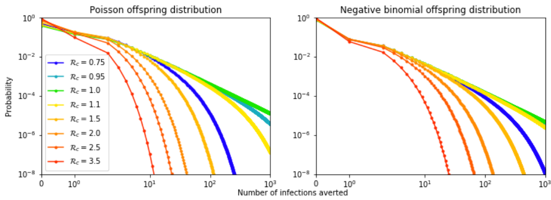
Figure 4: The distribution of the number of if a single individual isolates after infection. Calculated for Poisson and negative binomial distribution (with dispersion parameter 0.16). For R_c=1 the result is a power law distribution. If R_c is larger or smaller than 1, the distribution falls off quicker. For a given R_c , both distributions have the same mean, but the negative binomial distribution results in a more heterogeneous outcome (both 0 infections averted or many infections averted become more common in distributions with a heavier tail).
