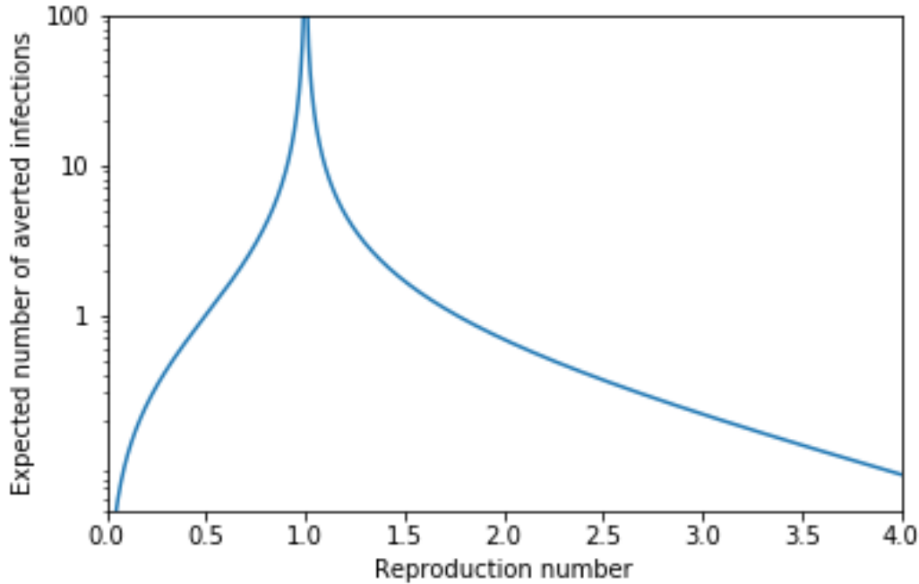
Figure 3 The expected number of averted infections, F(R_c) , due to a single infected individual isolating after infection and not transmitting, after accounting for overdetermination. The result is independent of the specific offspring distribution. This depends only on the average, R_c . Note the divergence to \infty as the reproduction number R_c \rightarrow 1 , and the decay to 0 as R_c decreases towards 0 or increases towards \infty .
