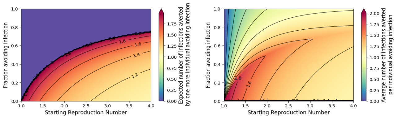
Figure 7: Measuring the impact of many individuals taking actions (such as a vaccine or prophylactic medication) to avoid infection without prior knowledge of whether they would be infected otherwise. Left: The marginal reduction in infections from one more individual changing behavior. The marginal benefit increases until the epidemic threshold is reached. Near the epidemic threshold, on average each additional individual acting prevents about 2 infections. Above the critical fraction avoiding infection (purple region), each additional individual has no net impact. Right: The number of infections averted over the entire population taking protective action. Until enough individuals take action to prevent an epidemic, the average is greater than 1, and the average increases until the threshold is reached after which it begins to fall.
