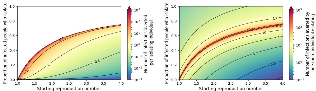
Figure 5: Measuring the effectiveness of many individuals isolating. Left The average impact assuming that other interventions set a starting value of R_c , but an additional fraction of the infected individuals isolate. Calculations are done in the limit of an infinite population. As the fraction of infections isolating increases, the size of the epidemic decreases. Eventually a larger fraction isolating translates to a smaller absolute number isolating due to the smaller epidemic. When enough isolate to drive the resulting R_c close to 1 almost all infections are averted while only a small fraction of the total population isolate, so the number of infections averted per isolating individual diverges. Beyond this threshold (white region), epidemics are impossible and the number of infections averted per infected individual is infinite. Right The marginal benefit of one more infected individual isolating. That is, given the fraction isolating and the initial R_c , this gives the number of infections averted if one additional infected individual who would not isolate is successfully identified and isolated.
