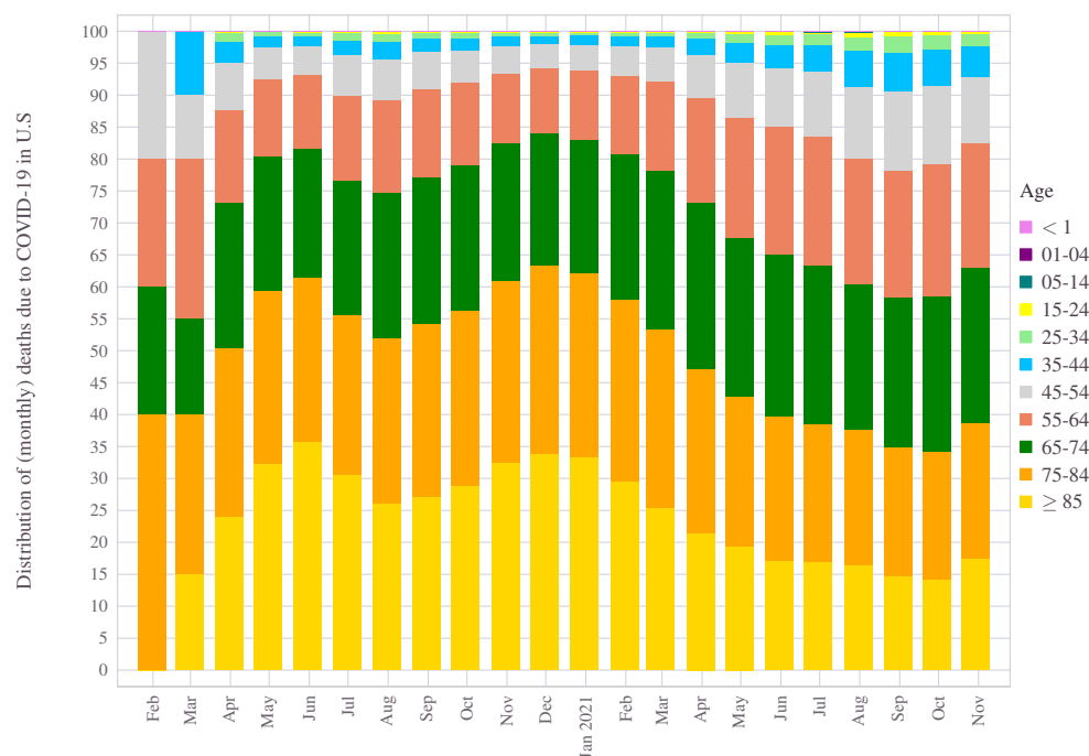
Figure 39. Vaccine impact: Change in the distribution of deaths across age profiles over time. Since the deployment of the vaccine, a noticeable improvement was seen in the mortality rates of oldest adults and gradually moving towards an equal distribution of deaths among broader sets of adult age groups.
