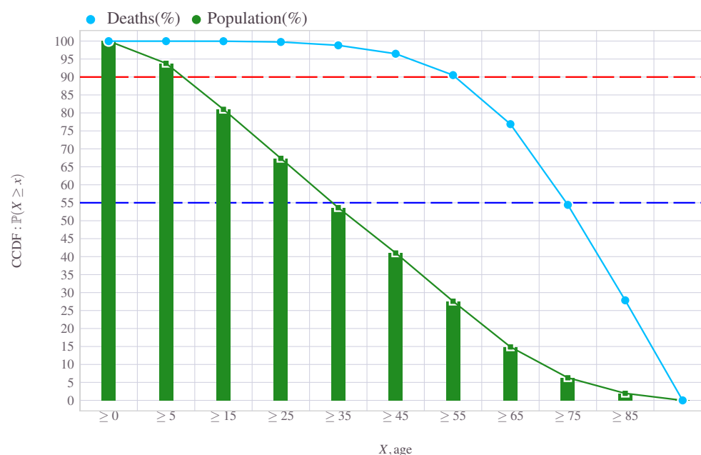
Figure 7. CCDF plot of Death and CCDF of Population, both distributed among age groups
