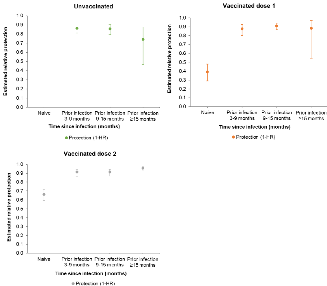
Figure 2: Protection following primary infection under different COVID-19 vaccination scenarios, up to 18 months following infection
