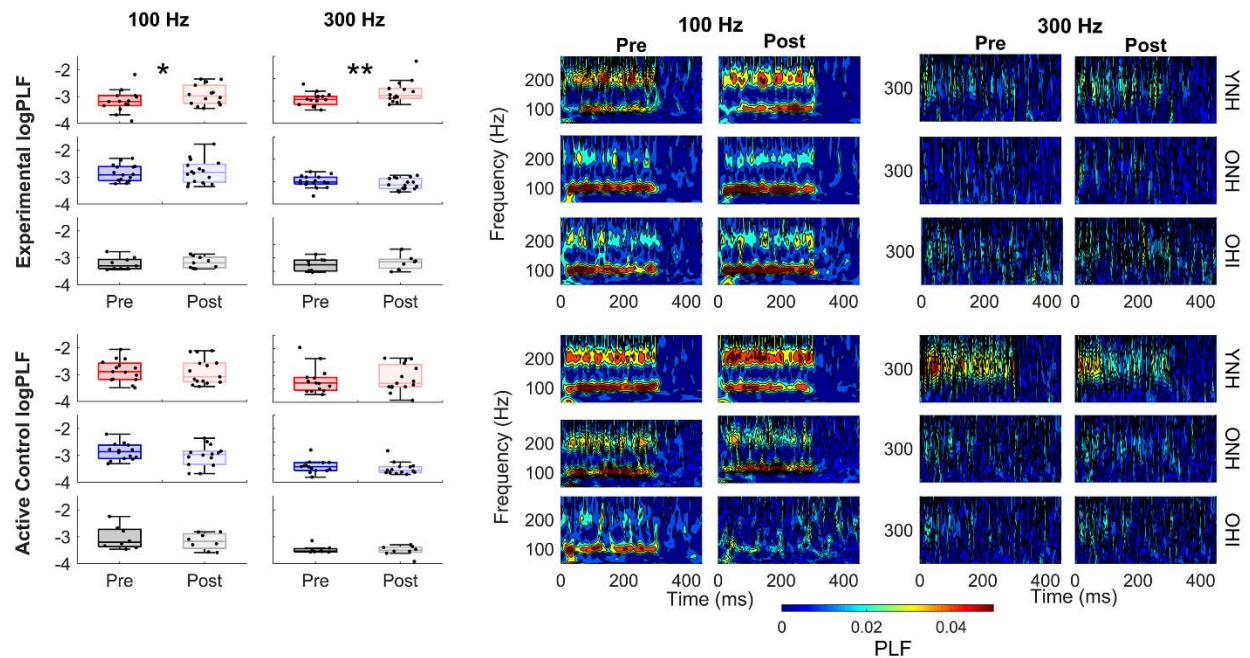
739 Figure 4. Pre- and post-training phase-locking factor (PLF) for 100- and 300-Hz rates is 740 displayed in box plots and in the time-frequency domain for young normal-hearing (YNH), older 741 normal-hearing (ONH), and older hearing-impaired (OHI) listeners in the experimental (top three 742 panels) and active control (bottom three panels) groups. Note that these values are log- 743 transformed. There were significant increases in PLF in the training group, especially in the 744 YNH listeners, that were not observed in the active control group. * P < 0.05 , ** P < 0.01 . 745 Medians: Inside box lines. Upper and lower quartiles: top and bottom edges of the box, 746 respectively. The endpoints of the whiskers represent the range of values without the outliers.
