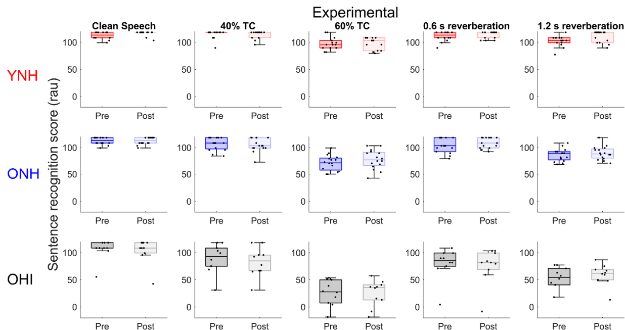
780 781 Figure 9. Active control. Box plots and individual data points displayed for rau-transformed 782 percent of correct items pre-and post-training for clean speech, 40% time-compressed speech 783 (40% TC), 60% time-compressed speech (60% TC), and 0.6 s and 1.2 s reverberation time in 784 young normal-hearing (YNH), older normal-hearing (ONH), and older hearing-impaired (OHI) 785 listeners in the active control group. No changes in performance were noted in any listener 786 group. Medians: Inside box lines. Upper and lower quartiles: top and bottom edges of the box, 787 respectively. The endpoints of the whiskers represent the range of values without the outliers. 788 Rau: rationalized arcsine transform
