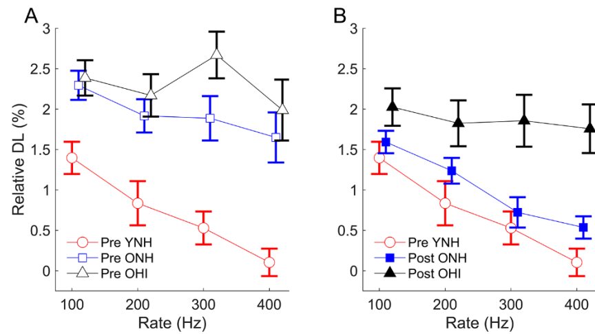
731 Figure 3. Relative DLs (log-transformed) are compared between young normal-hearing (YNH), 732 older normal-hearing (ONH), and older hearing-impaired (OHI) experimental training groups for 733 pre-test data (Panel A) and between pre-test YNH and post-test ONH and OHI groups (Panel B). 734 The pre-test differences between YNH and ONH groups were not present at post-test, but 735 differences persisted for the OHI groups. Errors bars: \pm 1 S.E.
