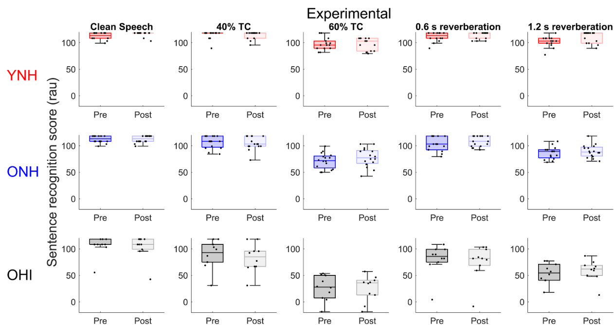
772 Figure 8. Experimental group. Box plots and individual data points displayed for rau-transformed 773 percent of correct items pre- and post-training for clean (undistorted) speech, 40% time- 774 compressed speech (40% TC), 60% time-compressed speech (60% TC), and 0.6 s and 1.2 s 775 reverberation time in young normal-hearing (YNH), older normal-hearing (ONH), and older 776 hearing-impaired (OHI) listeners in the experimental group. No changes in performance were 777 noted in any listener group. Medians: Inside box lines. Upper and lower quartiles: top and 778 bottom edges of the box, respectively. The endpoints of the whiskers represent the range of 779 values without the outliers. Rau: rationalized arcsine transform
