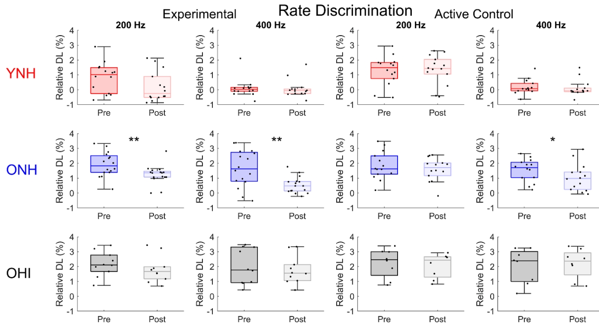
718 Figure 2. Rate discrimination at two untrained rates. Box plots and individual data points 719 displaying difference limens (DLs) as a function of 200- and 400-Hz rates obtained in young 720 normal-hearing (YNH), older normal-hearing (ONH), and older hearing-impaired (OHI) listeners 721 who completed nine sessions of rate discrimination training (experimental) or signal detection in 722 noise training (active control). Note that these percentages are log-transformed. There were 723 significant improvements in performance (decreased DLs) in the experimental group (especially 724 the ONH and OHI), that were not observed in the active control group (except for the ONH 400- 725 Hz rate). * P < 0.05 , ** P < 0.01 . Medians: Inside box lines. Upper and lower quartiles: top and 726 bottom edges of the box, respectively. The endpoints of the whiskers represent the range of 727 values without the outliers.
