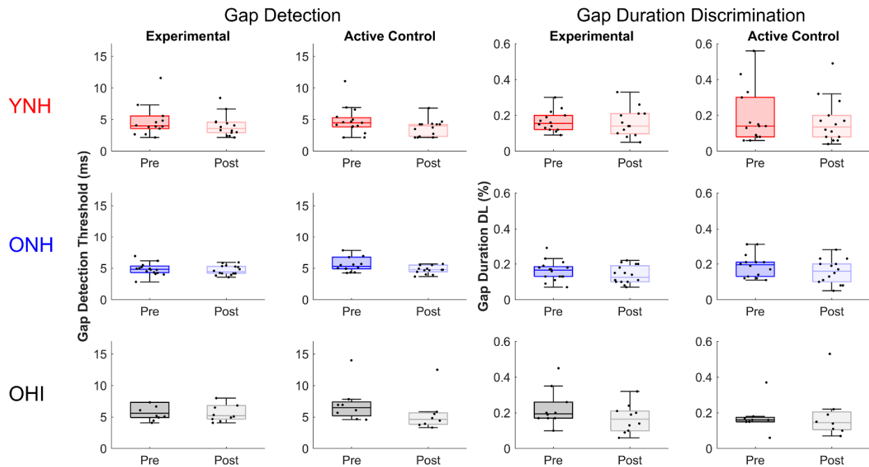
756 Figure 6. Pre- and post-training gap detection thresholds and gap duration DLs are displayed in 757 box plots and individual data points for young normal-hearing (YNH), older normal-hearing 758 (ONH), and older hearing-impaired (OHI) listeners in the experimental and active control 759 groups. No changes in performance were noted from pre-test to post-test in any group. Medians: 760 Inside box lines. Upper and lower quartiles: top and bottom edges of the box, respectively. The 761 endpoints of the whiskers represent the range of values without the outliers.
