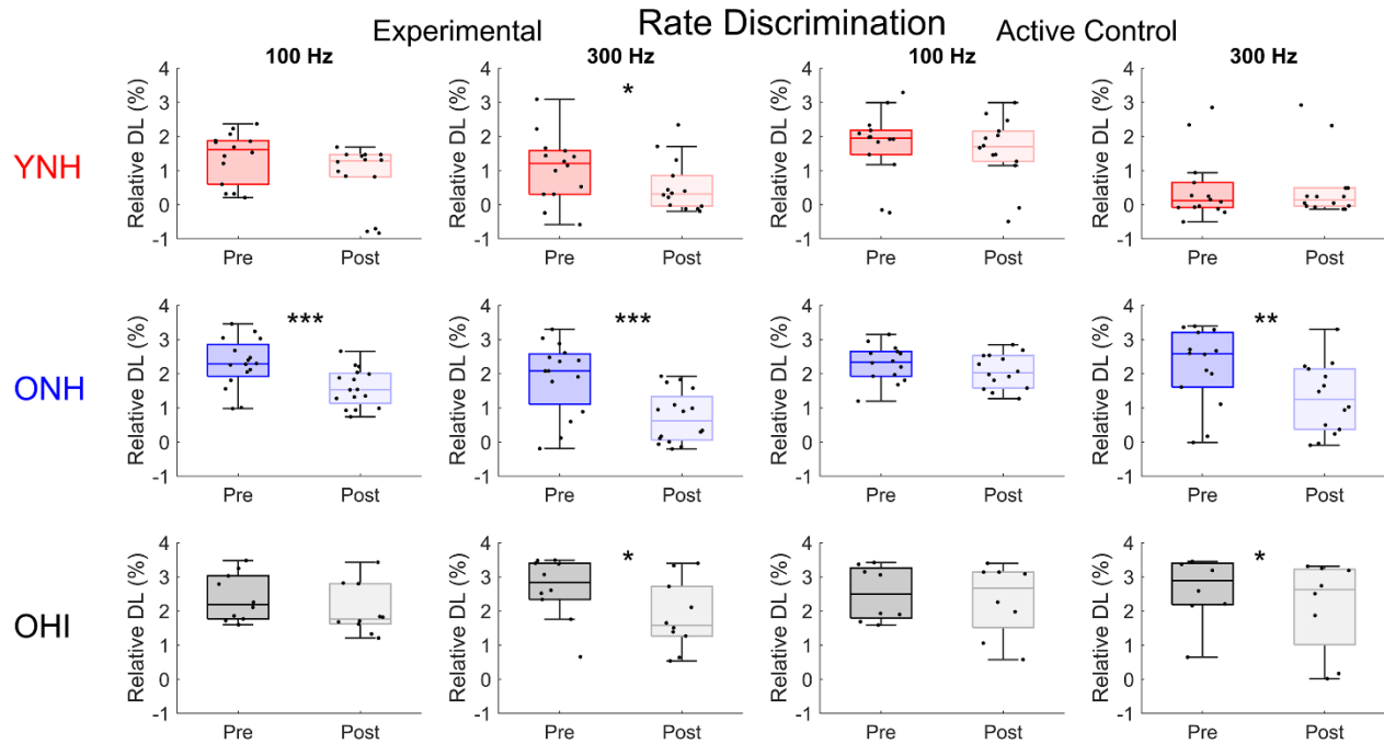
707 Figure 1. Rate discrimination at two training rates. Box plots and individual data points 708 displaying pre- and post-training relative difference limens (DL) as a function of 100- and 300- 709 Hz rates obtained in young normal-hearing (YNH), older normal-hearing (ONH), and older 710 hearing-impaired (OHI) listeners who completed nine sessions of rate-discrimination training 711 (experimental group) or tone-in-noise detection training (active control group). Note that these 712 percentages are log-transformed. There were significant improvements in performance (smaller 713 DLs) in the experimental group that were not observed in the active control group. *P < 0.05, **P 714 < 0.01, ***P < 0.001. Medians: Inside box lines. Upper and lower quartiles: top and bottom 715 edges of the box, respectively. The endpoints of the whiskers represent the range of values without the 716 outliers.
