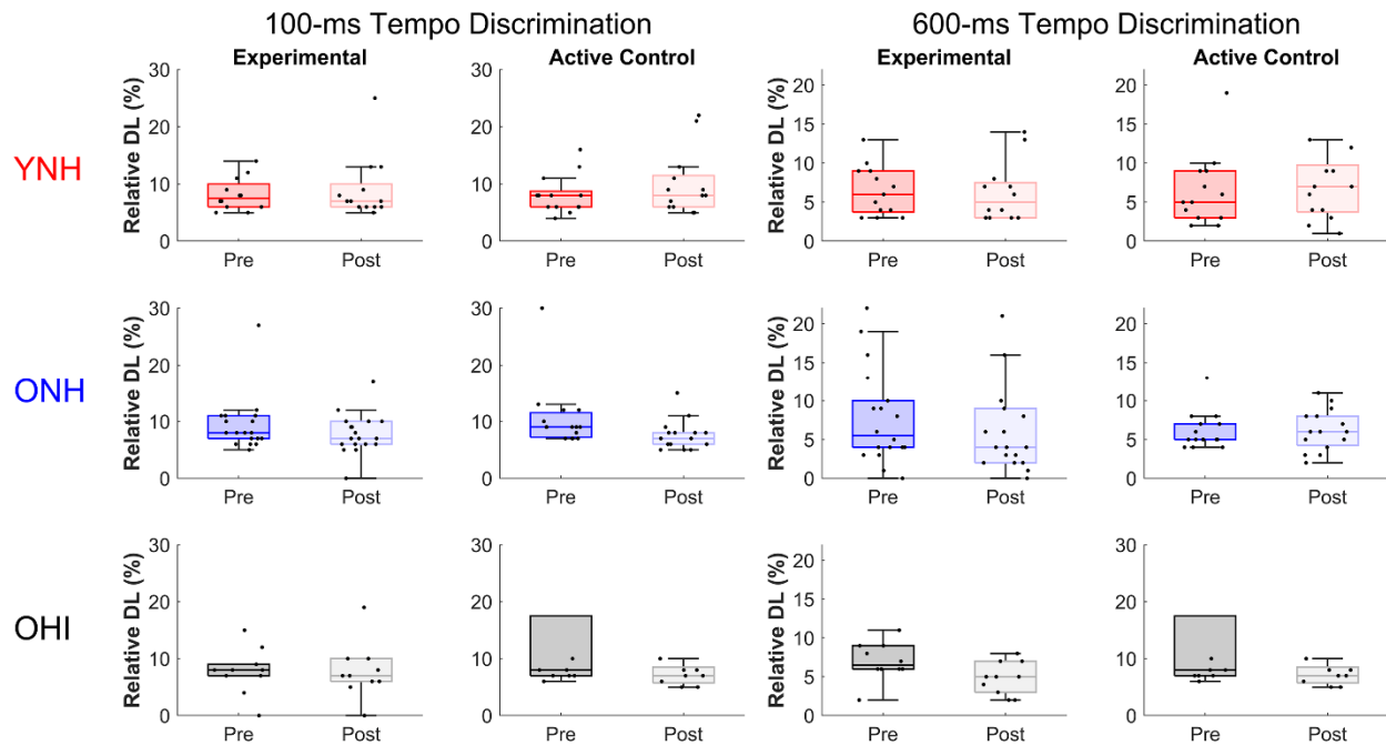
764 Figure 7. Box plots and individual data points for relative difference limens (DL) as a function of 765 100- and 600-ms inter-onset intervals (IOIs) obtained in young normal-hearing (YNH), older 766 normal-hearing (ONH), and older hearing-impaired (OHI) listeners in the experimental and 767 active control groups. No changes in performance were noted in any group. Medians: Inside box 768 lines. Upper and lower quartiles: top and bottom edges of the box, respectively. The endpoints of 769 the whiskers represent the range of values without the outliers.
