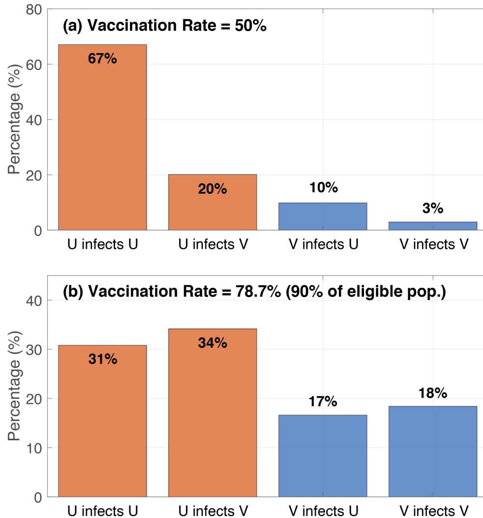
161 Figure 2: Likelihood that a new infection is caused by a (U) unvaccinated or (V) vaccinated individual 162 and that the new infection is in an unvaccinated or vaccinated individual. (a) shows a total vaccination 163 rate of 50%, where there are an equal number of vaccinated and unvaccinated individuals in the 164 population, while (b) shows a total vaccination rate of 78.7%, which is approximately the 90% eligible 165 population target. (a) also shows the expected result when normalizing by population.
