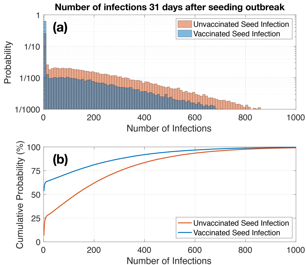
145 146 Figure 1: (a) Histograms showing probability of number of infections 31 days into an outbreak seeded by 147 (blue) one vaccinated individual or by (red) one unvaccinated individual. (b) Cumulative probability of 148 each number of infections for an outbreak seeded by (blue) one vaccinated individual or by (red) one 149 unvaccinated individual.
