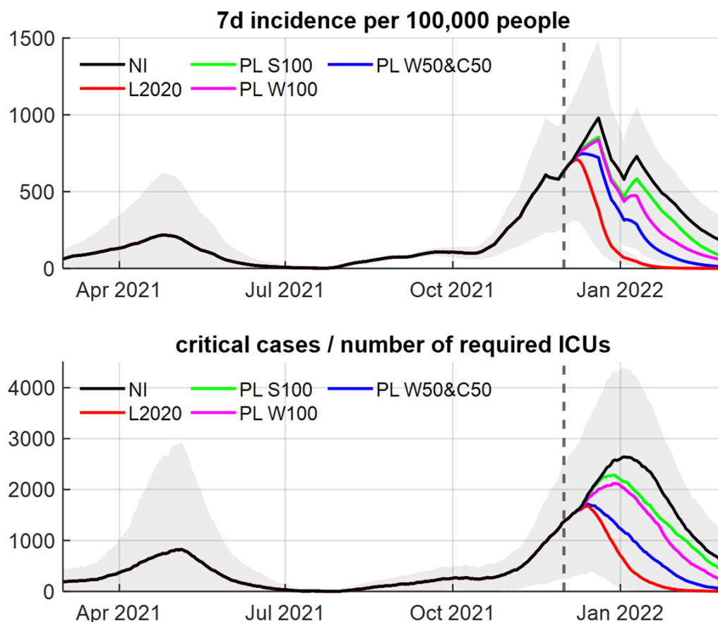
168 Fig. 2: The simulation results for the 7-day incidence and number of intensive care units required are shown. The 169 individual scenarios are colour-coded. Furthermore, the starting point of the interventions, 1 December 2021, is 170 also marked with a dashed line.
