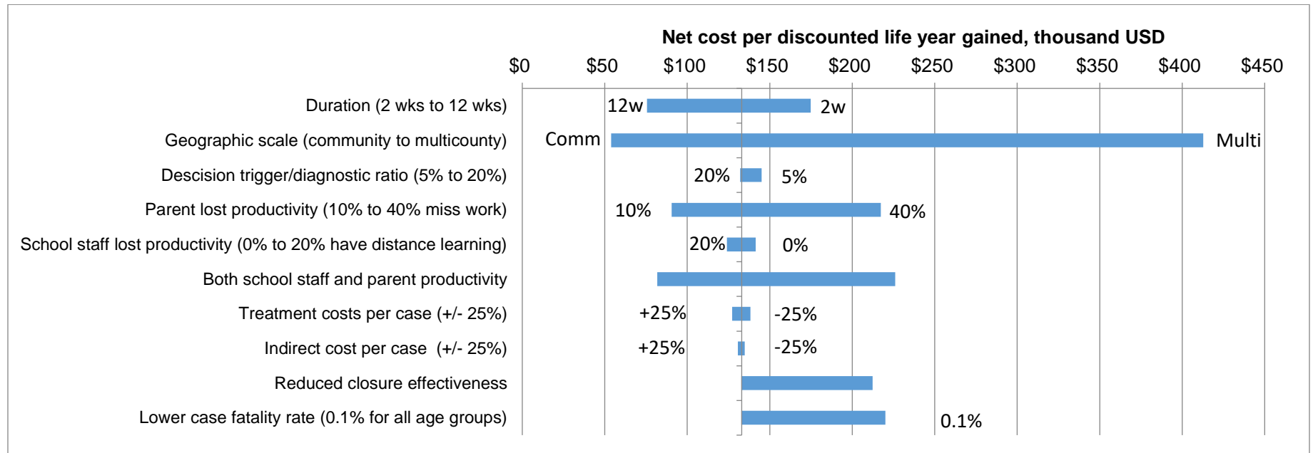
Figure 3d. One-way sensitivity analyses of the net cost per life-years gained relative to the 4-week county-level closure with a 10% diagnosis ratio assumption* at base-case values
