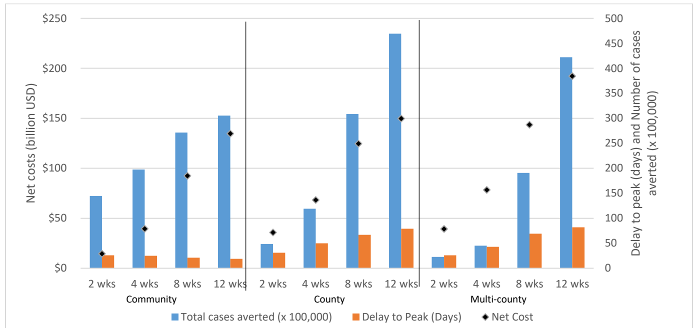
Figure 1a. Effect of increasing the duration of school closures (while keeping constant the geographic scale of school closures) on cases averted, delay to peak, and net cost for a national-level strategy against an influenza pandemic similar to the 1957 pandemic*
