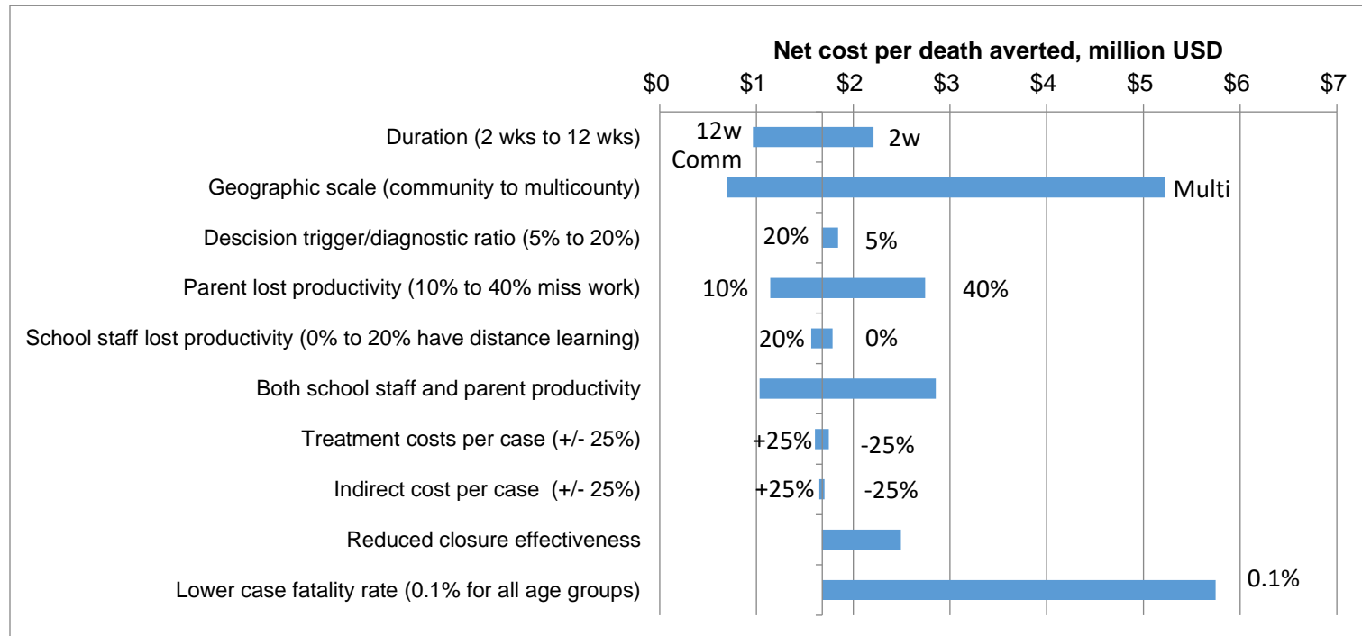
Figure 3c. One-way sensitivity analyses of the net cost per death averted relative to the 4-week county-level closure with a 10% diagnosis ratio assumption* at base-case values
