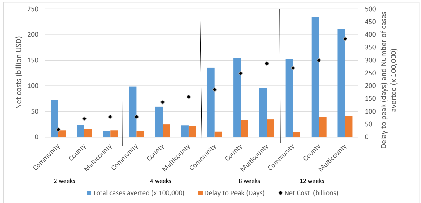
Figure 1b. Effect of increasing the geographic scale of school closures (while keeping constant the duration) on cases averted, delay to peak, and net cost for a national-level strategy against an influenza pandemic similar to the 1957 pandemic*
