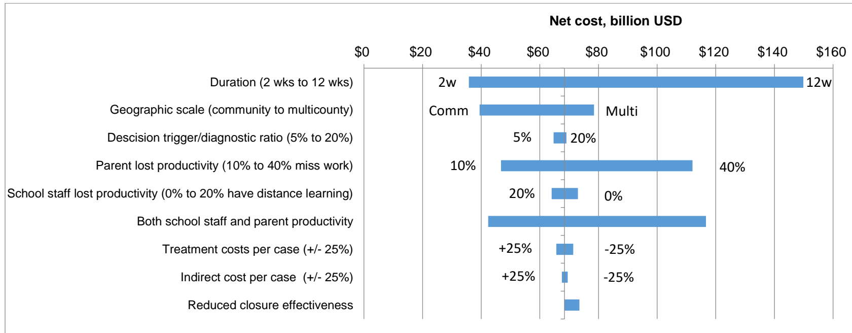
Figure 3a. One-way sensitivity analyses of the net cost of school closure to the 4-week county-level closure with a 10% diagnosis ratio assumption* at base-case values
